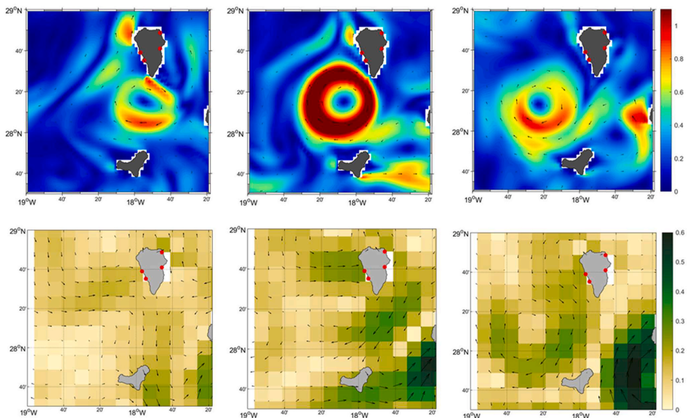
Fig. 7. Upper panels: Ocean velocity and intensity ( \text{m}\cdot\text{s}^{-1} ) at the near surface during June 28 th (left), July 10 th (middle) and July 23 rd of 2020 (right). Lower panels: Geostrophic velocity and intensity ( \text{m}\cdot\text{s}^{-1} ) at surface obtained from altimetry observations during the same dates.
