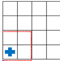
Figure 3.1.1. Schematic of the standard grid (black: 0.25 \times 0.25^\circ ), the large block (dashed red line) in which the grid origin is randomized. The cross (blue) shows the position where the origin of the grid is positioned to present the final results.
