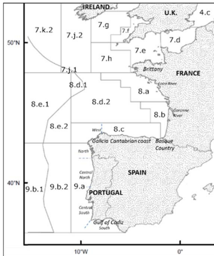
Figure 1.1. ICES divisions and subdivisions in southern Europe.
