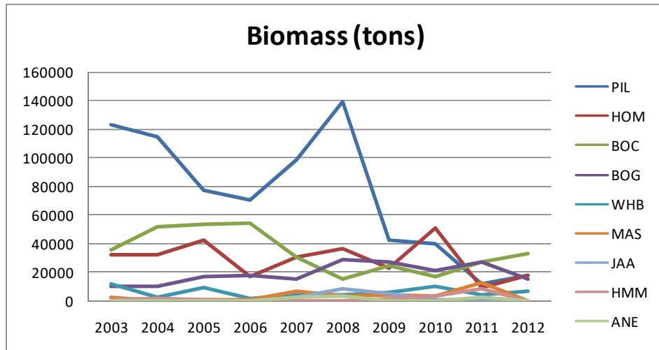
Figure 2.2.22. Biomass (tonnes) estimated for nine pelagic species during the 2003–2012 pelagic surveys.
