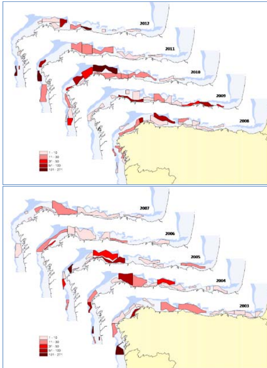
Figure 2.2.21. Mackerel spatial distribution during PELACUS (top, 2008–2012 cruises; bottom, 2003–2007 cruises). Polygon colours indicate the mean backscattering energy range ( s_A values, m^2 nmi^{-2} , 1–10; 11–30; 31–50; 51–100; and >100).
