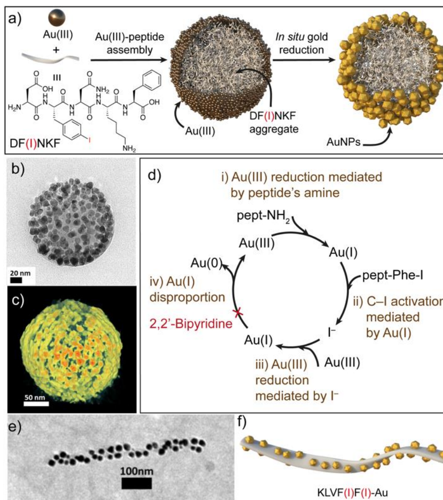
Fig. 3. a) Schematic representation of the formation of spherical DF(I)NKF-Au hybrid superstructures. b) TEM image and c) electron tomography reconstruction of DF(I)NKF-Au superstructures. d) Representation of the gold reduction mechanism. e) TEM image and f) schematic representation of helical KLVF(I)F(I)-Au superstructures. Adapted with permission from reference 37.
