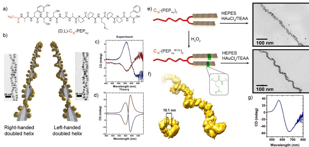
Fig. 6. a) Chemical structure of (D,L)-C 12 -PEP Au peptide conjugates. b) Schematic representation of the left- and right-handed superstructures and their corresponding TEM images. c) Experimental and d) theoretical CD spectra of the left- and right-handed superstructures. Adapted with permission from reference 35. Copyright 2013 American Chemical Society. e) Schematic representation of C 18 -(PEP Au ) 2 and C 18 -(PEP Au M-Ox ) 2 peptide conjugates and TEM images of their corresponding hybrid superstructures. f) Electron tomography reconstruction of the C 18 -(PEP Au M-Ox ) 2 single helical superstructures, and g) their CD spectrum. Adapted with permission from reference 70. Copyright 2016 American Chemical Society.
