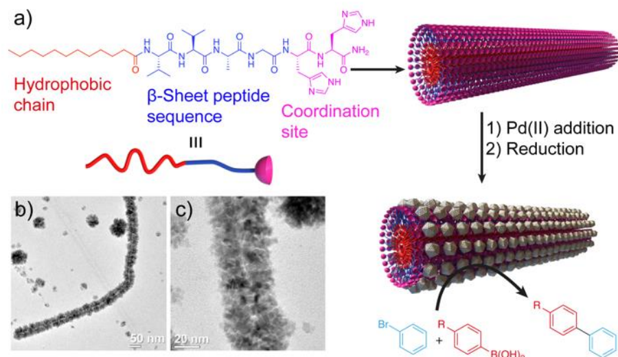
Fig. 9. a) Peptide chemical structure and schematic representation of the formation mechanism of the hybrid structures, which work as catalysts in Suzuki reactions. b) and c) TEM images of the resulting superstructures. Adapted from reference 57 with permission from the Royal Society of Chemistry.
