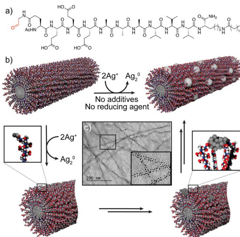
Fig. 4. a) Chemical structure of the peptide-amphiphile. b) Schematic representation of the proposed mechanism for the formation of peptide-AgNP hybrid nanofibres. c) TEM image of the hybrid nanofibres. Adapted with permission from reference 36.
