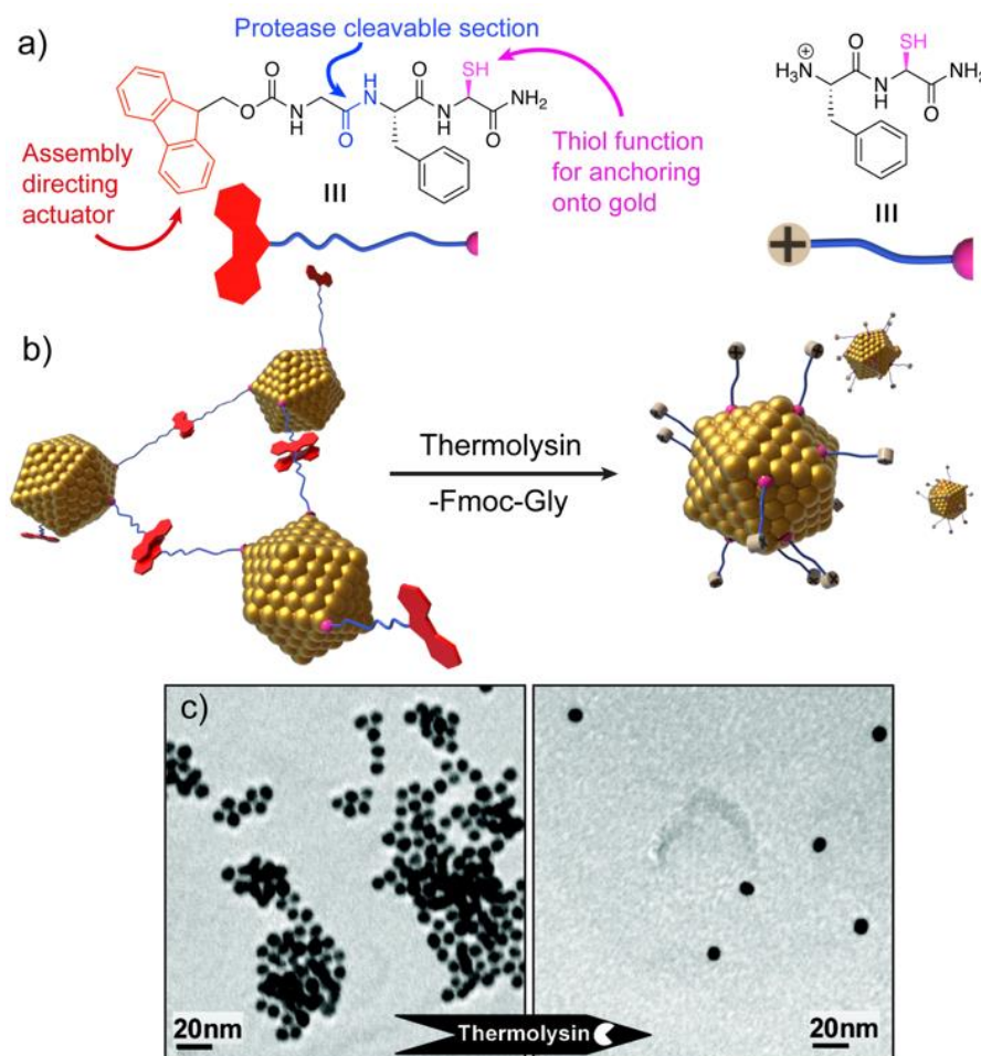
Fig. 7. a) Chemical structure and schematic representation of the peptide fragments. b) Schematic representation of the disassembly mechanism. c) TEM images of peptide-AuNP systems before and after exposure to protease. Adapted with permission from reference 78. Copyright 2007 American Chemical Society.
