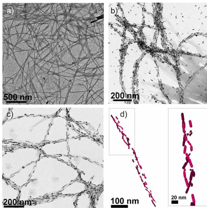
Fig. 10. a) TEM image of \alpha -synuclein fibrils. b) and c) TEM images of \alpha -synuclein fibrils in the presence of AuNRs at 2 and 0.5 nM concentrations, respectively. d) Cryo-TEM tomography reconstruction image showing a 3D chiral arrangement of the AuNRs. Reproduced with permission from reference 121.
