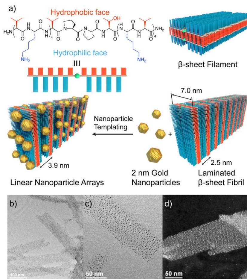
Fig. 5. a) Chemical structure of the amphiphilic peptide and schematic representation of the formation of the hybrid architectures. b) and c) TEM images, and d) high resolution TEM image showing the conserved spacing between AuNPs arrays. Adapted with permission from reference 64.
