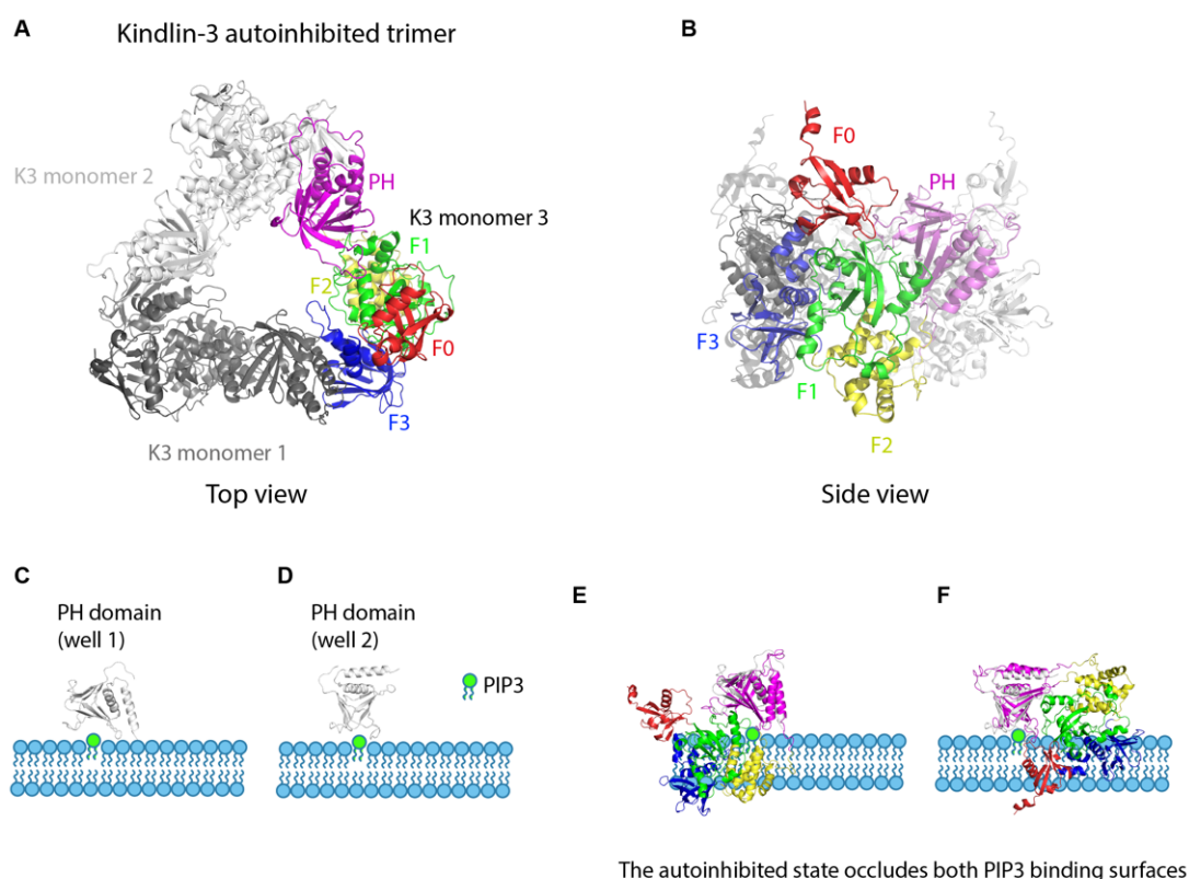
The autoinhibited state occludes both PIP3 binding surfaces
