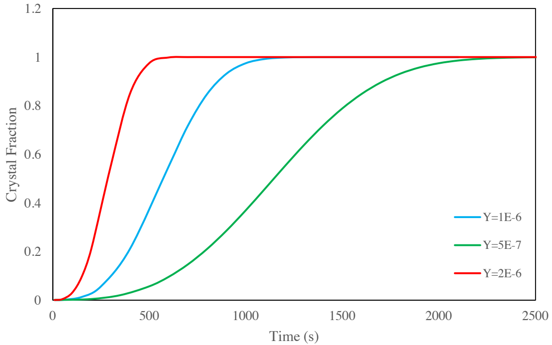
Figure 85. Avrami function calculated for different growth rates, with the same nucleation rate ( I=2.6 \times 10^{15} m^3/s )
