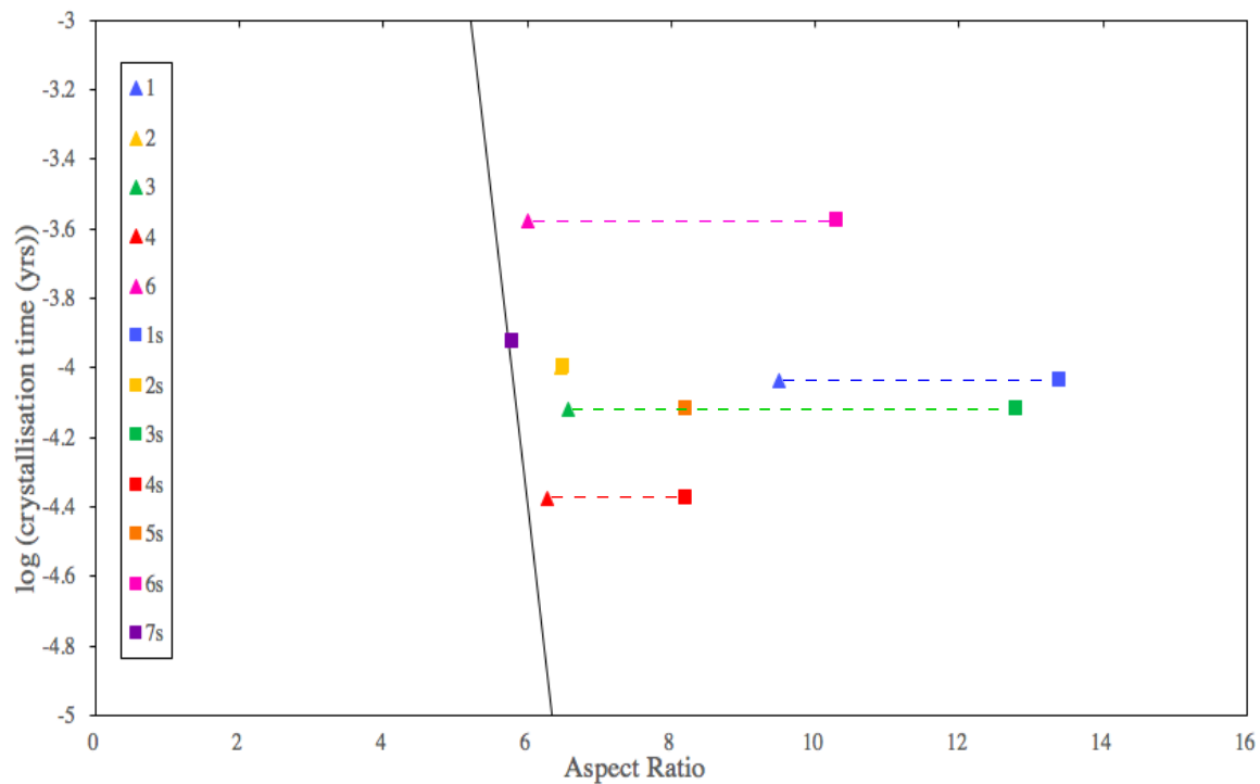
Figure 51. Data from the experiments done in this study compared to the equation and line derived in Holness (2014), for both SEM (squares) and microscope (triangles) measurements. Pairs of datasets for the same run are linked by the dotted lines, highlighting the difference between the datasets. The mean aspect ratio of experiment 2 was the same for both SEM and microscope measurements.
