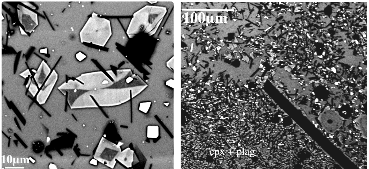
Figure 46. Backscattered electron images showing morphologies of clinopyroxene in sample 7 – regular octagonal sections (left) and dendritic (right). The image on the right also shows cpx growing around the edges of a larger pre-existing plagioclase crystal
