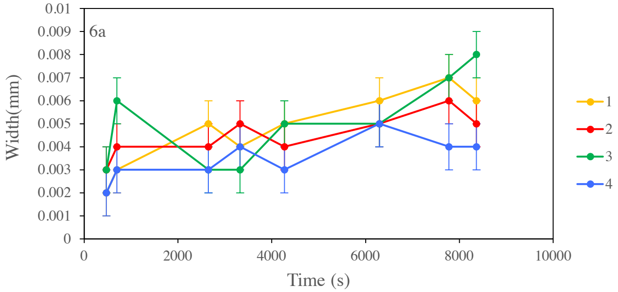
Figure 64. Plot of the changing widths over time of the individually tracked crystals from run 6, area A. Error bars represent error of 1 μm on measurements.
