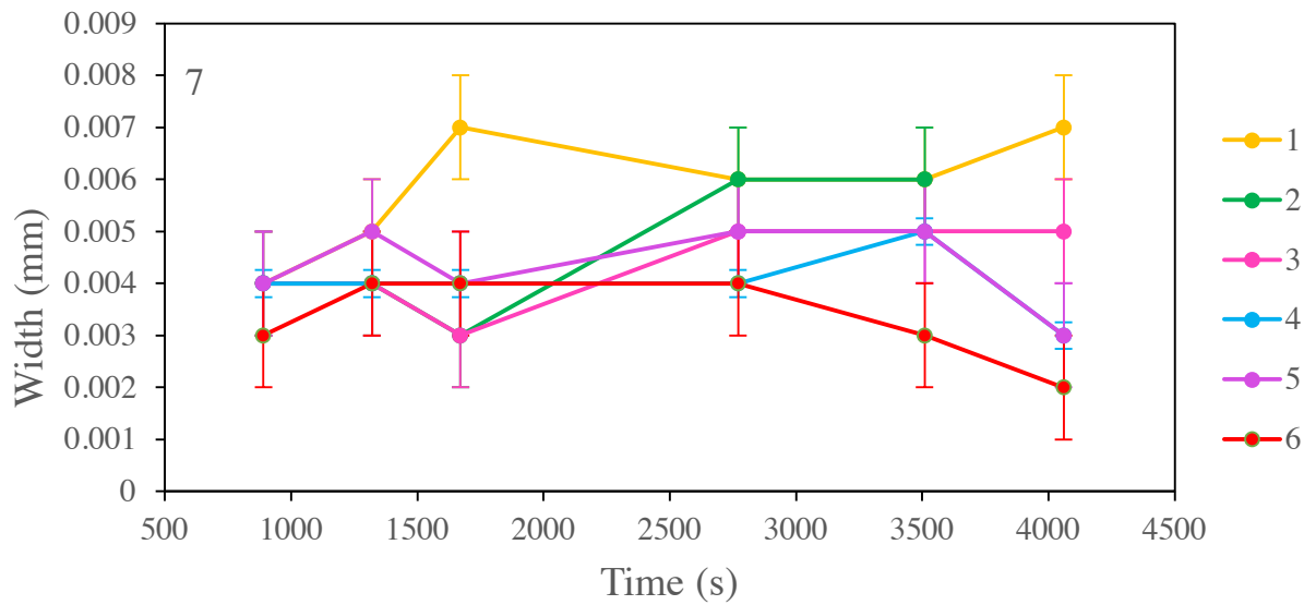
Figure 77. Plot of the changing width over time for the individually tracked crystals from run 7. Error bars represent measurement uncertainty of 1\mu\text{m}
