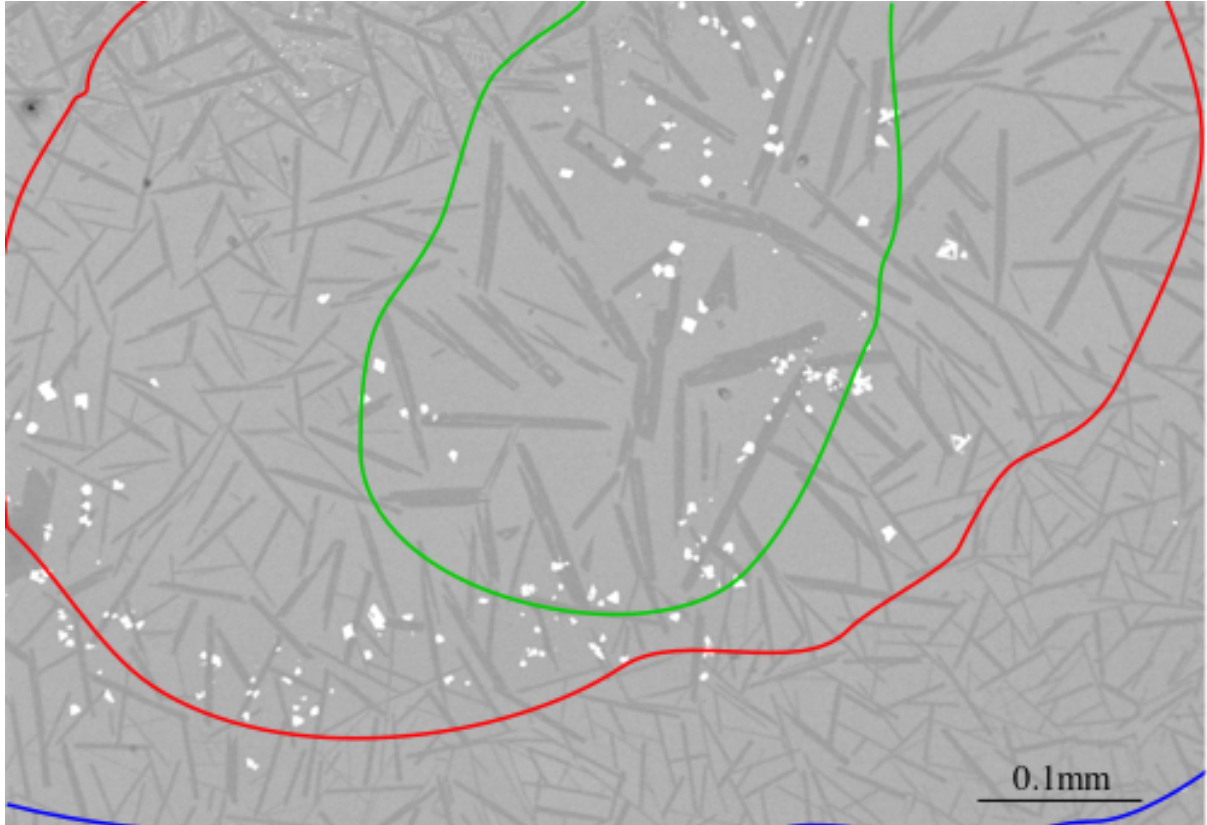
Figure 33. Backscattered electron image showing the general texture of the quenched sample after the first experimental run, with the zones used in figure 33 drawn on to outline the 3 different crystal size categories. It is possible that this variation was caused by sample thickness.
