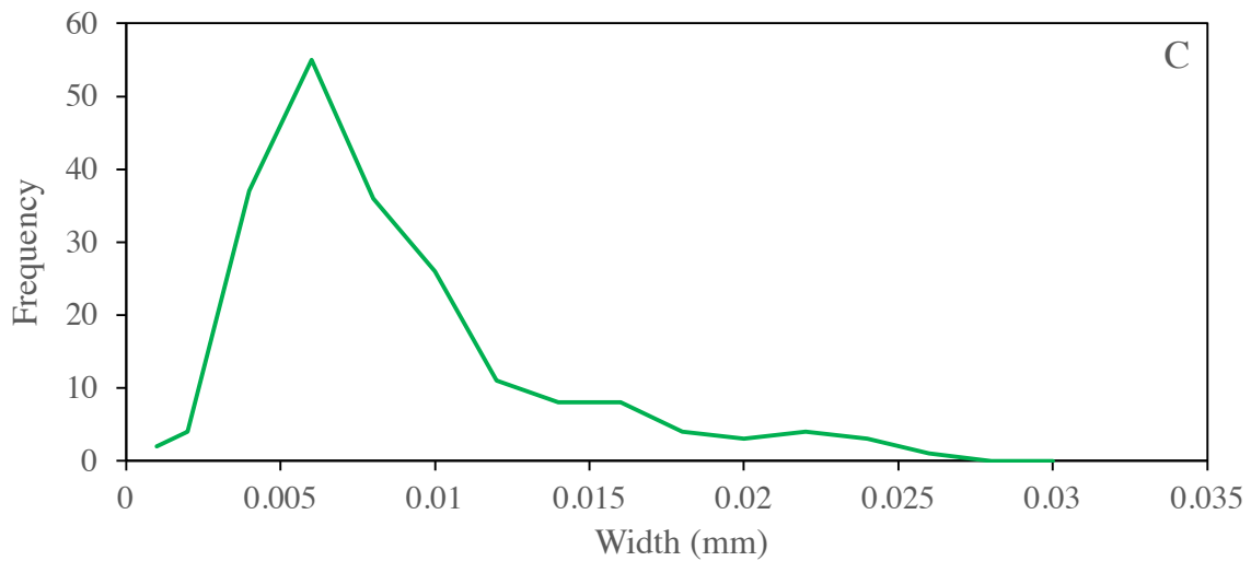
Figure 23. A-C, Frequency plots of plagioclase crystal aspect ratio (A), length(B) and width(C) from the BGP sample. Uncertainty in the length and width measurements is 1.1 \mu\text{m} , whilst average uncertainty in the aspect ratio measurements is 1.7.
