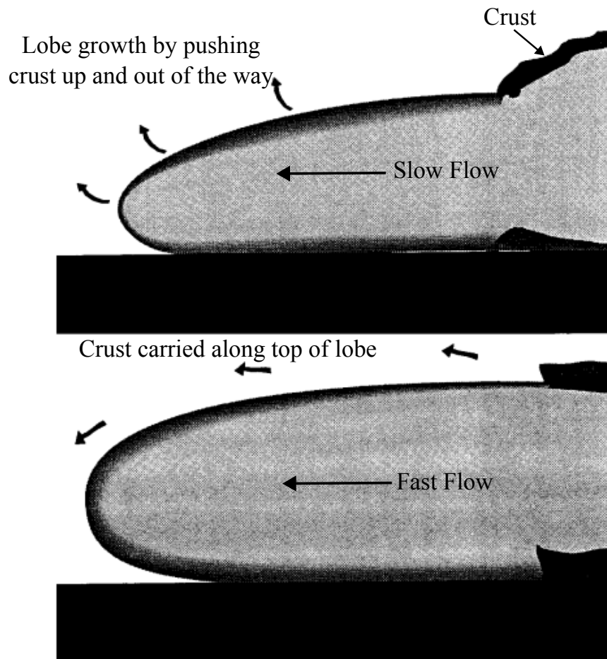
Figure 3.. Differences in pahoehoe lava flow lobes. Adapted from Keszhelyi and Denlinger (1995)
