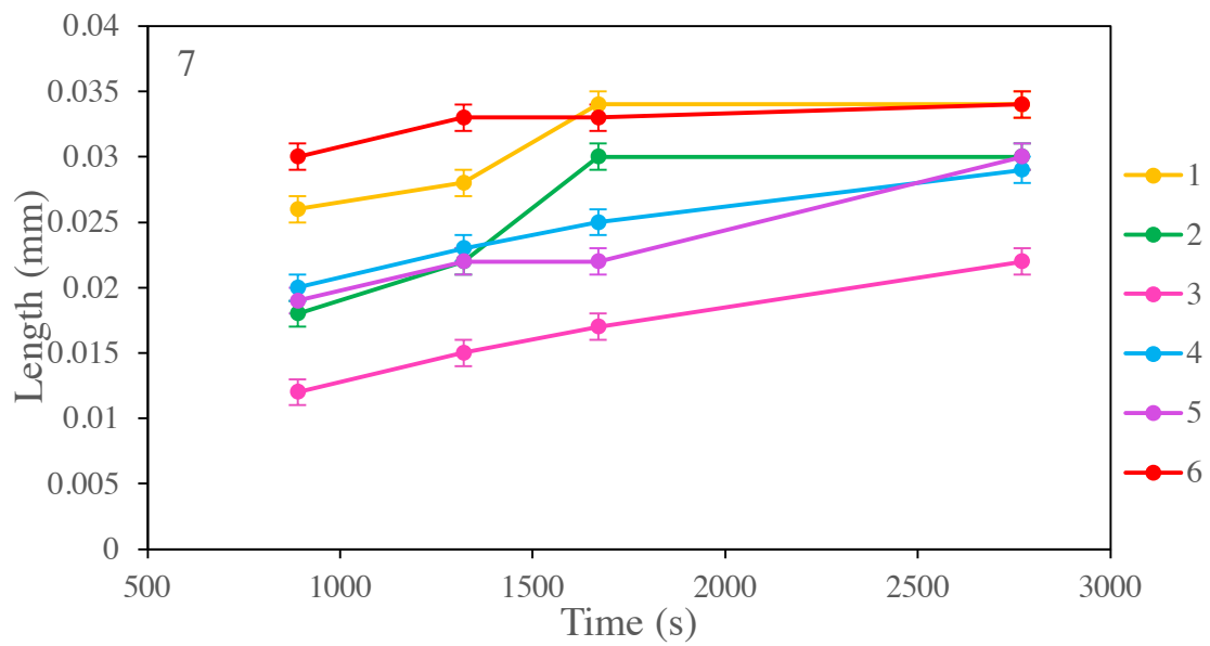
Figure 76. Plot of the changing length over time for the individually tracked crystals from run 7. Error bars represent measurement uncertainty of 1\mu\text{m}
