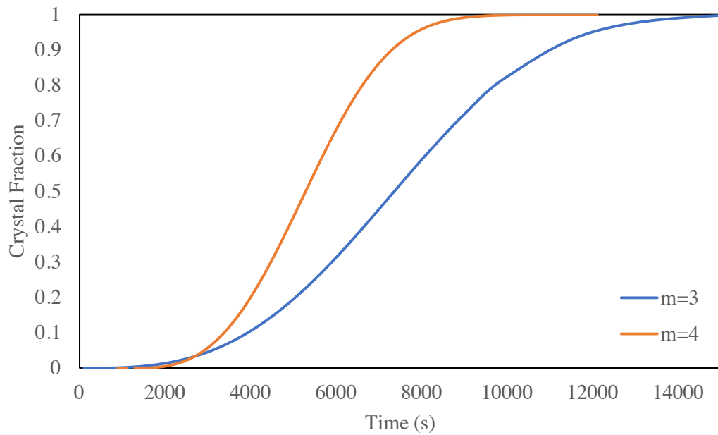
Figure 86. Avrami function calculated for the two different limiting forms, m=3 or 4 , with all other inputs kept the same ( I=1.6 \times 10^{-6} m^3/s , Y=2.2 \times 10^{-6} cm/s ).
