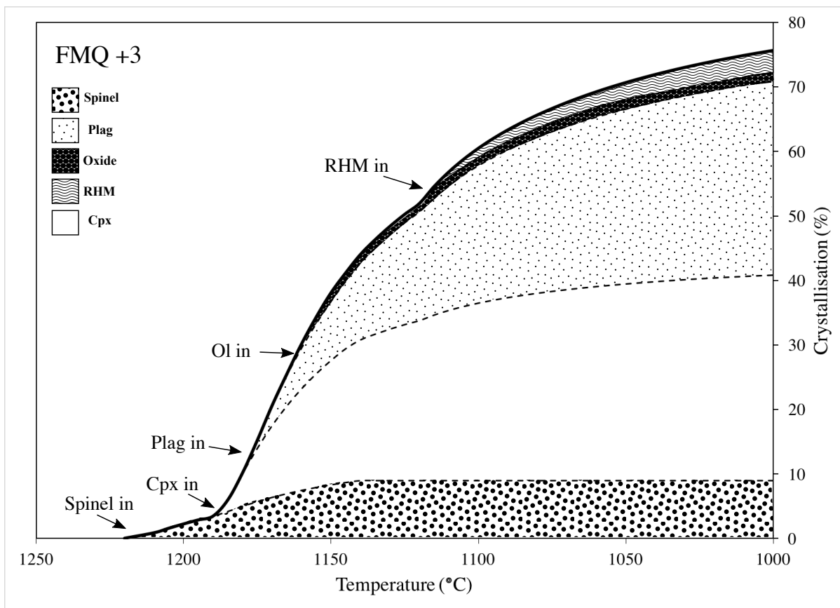
Figure 8a-b. Plot of phase growth with temperature from MELTS, from BGP melt for two contrasting fugacities (FMQ -1 (a) and +3(b)),
