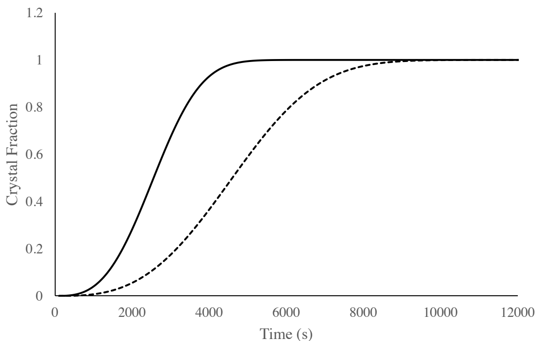
Figure 84. Avrami function calculated using the measured Y and N_v ( I=2.6 \times 10^6 ) for run 6 (solid line), and the same conditions but with a I recalculated and ‘corrected’ for the measured timescale of the experiment ( I=1.8 \times 10^6 ) (dashed line).
