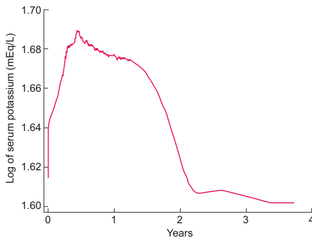
FIGURE 3: Trajectory of potassium measurements (transformed by its logarithm) along the entire follow-up period. The adjusted association with time (years) was highly significant (overall P-value for the trajectory <0.0001). The values were lower in the initial visit and corresponded to a patient's evaluation before the admission for hyperkalaemia. The zenith of potassium was found during the acute episode in the emergency room. Afterwards, we found a progressive and significant decrease in the potassium levels during follow-up.
