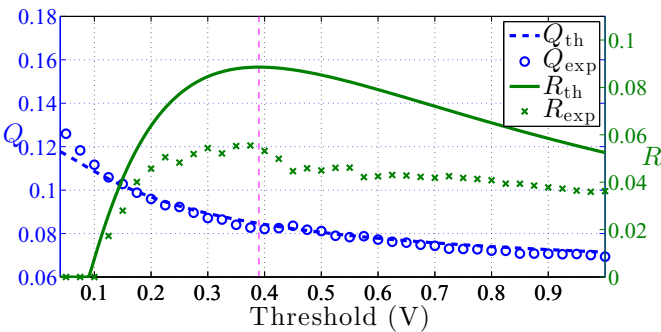
FIG. 5. (Color online) Experimental QBER ( Q_{exp} ) and secure key rate ( R_{exp} ) in functions of the probe threshold (measured by the photodiode voltage). Dashed and solid lines show the corresponding theoretical predictions ( Q_{th} and R_{th} , respectively).
