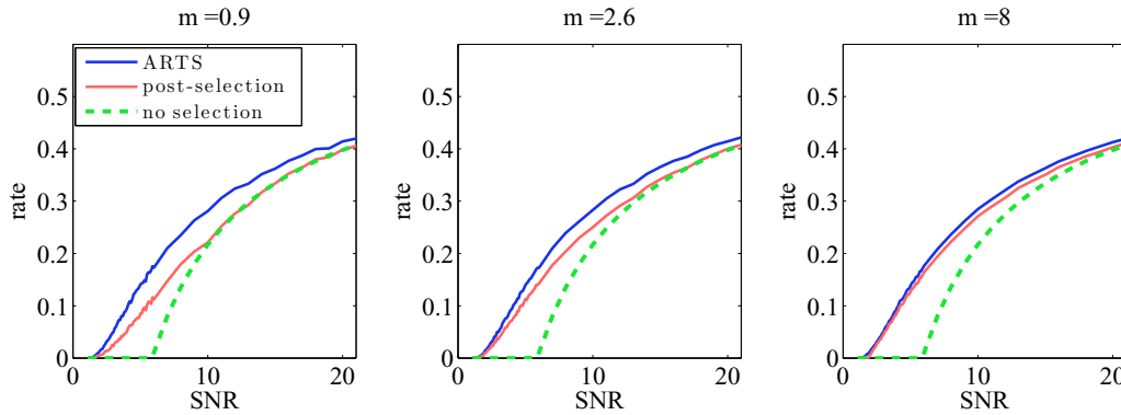
FIG. 6. (Color online) Comparison between the rates achievable by the ARTS, the postselection, and the standard QKD technique (no selection). We assumed that the channel QBER is 3% and the log-normal parameter is \sigma = 1 , similar to the parameter we measured in the tested free-space channel. The parameter m represents the mean received bits per coherence time of the channel.
