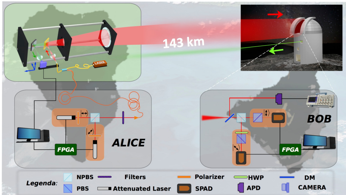
FIG. 1. (Color online) Experimental setup: Alice is located at JKT observatory in La Palma. Qubits are prepared using a field-programmable gate array (FPGA) controller, linear optical components, and attenuated lasers. Alice telescope is also configured to acquire the beacon beam sent by Bob, located at the Optical Ground Station in Tenerife, and used for tracking the transmitter in order to stabilize the pointing.
