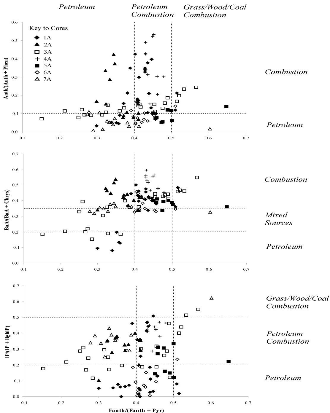
Figure 8. PAH isomeric cross-plot of sediments from Clyde Estuary for the determination of PAH origin. Abbreviations: Anth=Anthracene; Phen=Phenanthrene; BaA=Benz[a]anthracene; Chrys=Chrysene; IP=Indenol[1,2,3- cd ]pyrene; BghiP=Benzo[ ghi ]perylene.
