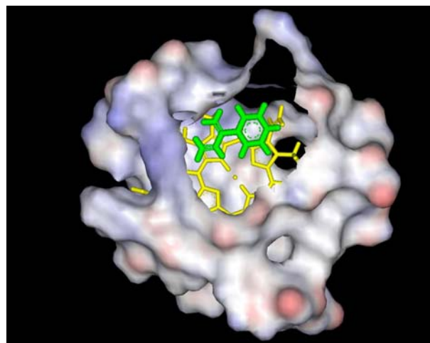
Fig. 4 Surface representation of model (S315R) structure with heme (Yellow colored) and INH (Green colored) docked into the cavity
