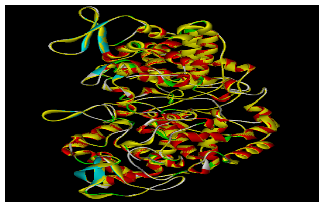
Fig. 2 (d) Superimposed model of template and the target. 1S2J-WT template (Yellow colored) KatG-mutant target (Red colored) models were viewed in Rasmol (V-2)
