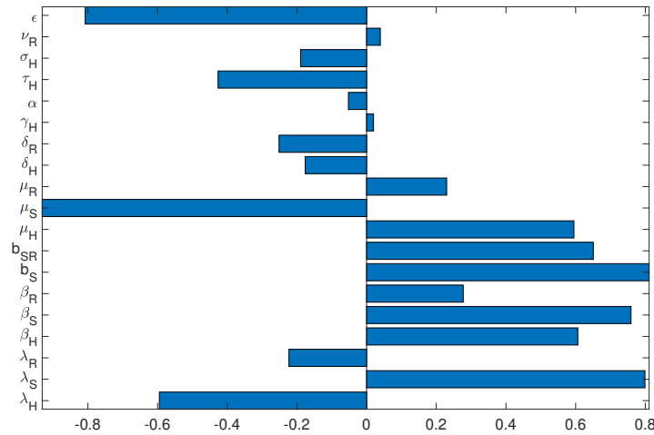
FIGURE 2. PRCC values for the leishmaniasis model (2.1), using the reproduction number ( \mathcal{R}_0 ) as the response function. Parameter values (baseline) and ranges used are as given in Table 2.
