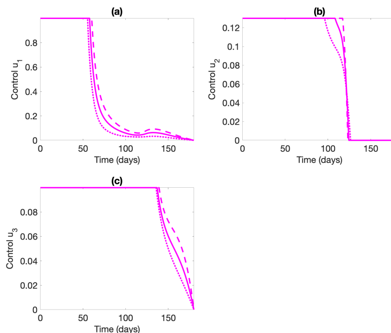
FIGURE 6. Optimal controls of the leishmaniasis model (4.1) in the \pm 50\% uncertainty interval of parameters \Lambda_R, \Lambda_S and b_{SR} for: (a) Personal protection control; (b) Sandflies insecticide control; (c) Reservoir culling control. The parameters \Lambda_R, \Lambda_S and b_{SR} are set within \pm 50\% interval of their baseline values given in Table 2 and all other parameters are taken in their baseline values. In all plots, the solid curves represent the plot for baseline values of all parameters, the dotted curves represent the plot for lower bound of the three parameters and the dashed curves represent the plot for upper bound of these three parameters.
