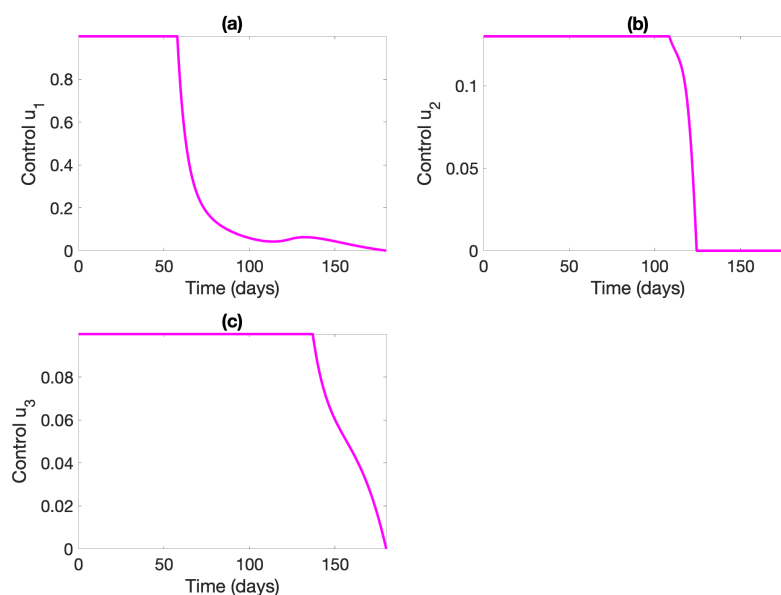
FIGURE 4. Optimal controls of the leishmaniasis model (4.1) for: (a) Personal protection control; (b) Sandflies insecticide control; (c) Reservoir culling control.
