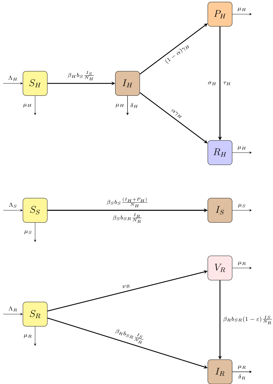
FIGURE 1. Systematic flow diagram of model (2.1).
