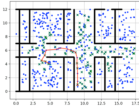
Figure 10: Path from the initial location of robot r2 to room 6 found using PRM
