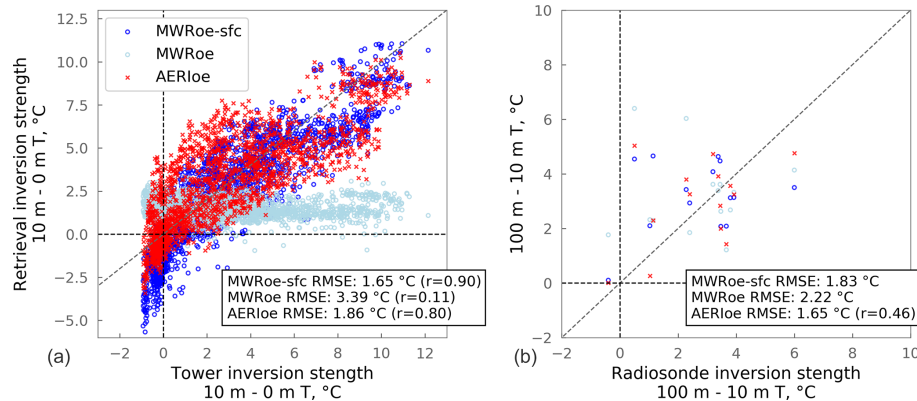
Figure 6. (a) Inversion strength (10–0 m temperature, T ) retrieved from the AERloe (red), the MWRoe (light blue), and the MWRoe-sfc (dark blue) versus observations from the tower-mounted HMP155 probes. (b) The same as (a) except for the 100–10 m inversion strength compared to observations from 14 coincident radiosonde profiles. On both subplots, the diagonal grey dashed line represents perfect agreement, and the horizontal and vertical dashed black lines at 0 °C delineate when a surface-based temperature inversion is present (right quadrants) versus absent (left quadrants). The root-mean-squared error (RMSE) values are included on the plots, and the Pearson's correlation coefficients ( r ) are only included when they are significant at the 90 % confidence level.
