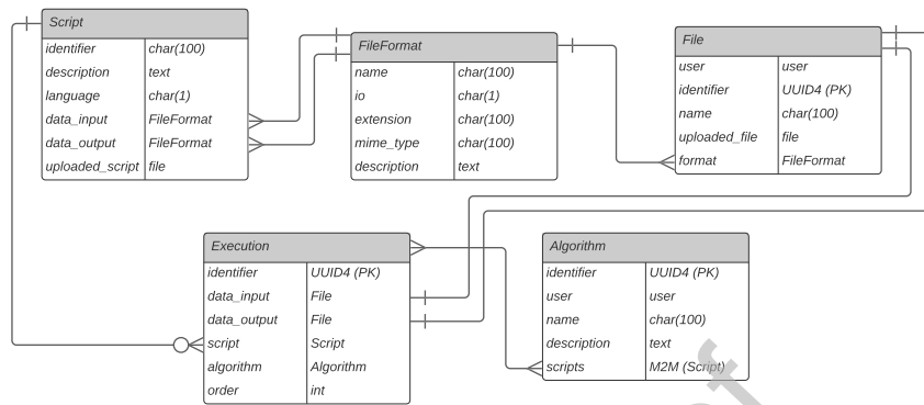
Figure 1: Entity relationship diagram (ERD) of the algorithm development database. Each table represents a model in the Django framework. 'Algorithm' is the user-created entry consisting of a list of 'Scripts' which process 'Files' in the order set by 'Execution' providing they are a compatible 'FileFormat'
