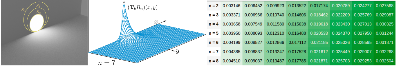
Fig. 3. Illustration of our proof that the radiant exitance transport operator T_b is not compact. Left : rendered scene with a disk S_n emitting diffuse light. The disk is tangential to the abutting edge. Center : measured radiant exitance on the receiver surface for n = 7 . As n is increased, the spatial frequencies of the emitted energy increases while preserving its L_2 norm, as does the received energy. In the limit, it escapes any finite rank approximation over the space of functions on the receiver. Right : table showing that the pairwise measured L_2 distances between T_b B_n and T_b B_{n+p} do not depend on n (for large n , because the receiver is bounded) and converges to non-zero values with p for a given n . To ensure numerical accuracy in this figure we reduce the disk radius by a factor of 1.2 instead of 2, and use the analytical formula of Naraghi [1988].
