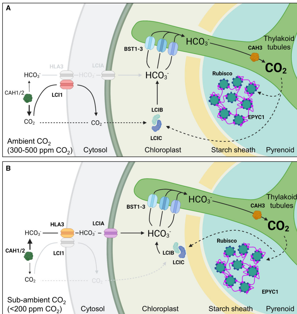
Figure 1 Overview of inorganic carbon uptake in the Chlamydomonas CCM. A, At ambient levels of \text{CO}_2 (300–500 ppm, 0.03–0.05%, 10–18 \mu\text{M} \text{CO}_2 ), extracellular inorganic carbon (Ci, i.e. \text{CO}_2 and hydrated Ci, such as \text{HCO}_3^- ) uptake is thought to be driven by drawdown of \text{CO}_2 into the chloroplast through rapid conversion of \text{CO}_2 to bicarbonate ( \text{HCO}_3^- ) by LCIB, which is dispersed throughout the stroma in a complex with LCIC. \text{HCO}_3^- is then transported into the lumen of thylakoid tubules traversing the pyrenoid by bestrophin-like channels (BST1-3) on the pyrenoid periphery. Carbonic anhydrase 3 (CAH3) located in the lumen within the pyrenoid converts \text{HCO}_3^- to \text{CO}_2 , which diffuses into the surrounding Rubisco-EPYC1 matrix. \text{CO}_2 not assimilated by Rubisco is converted back to \text{HCO}_3^- by LCIB. Periplasmic carbonic anhydrases 1 and 2 (CAH1/2) and the plasma membrane \text{CO}_2 channel low \text{CO}_2 -inducible protein 1 (LCI1) assist with inward \text{CO}_2 diffusion (Fujiwara et al., 1990). Font sizes for \text{CO}_2 and \text{HCO}_3^- represent their relative concentration. B, At sub-ambient \text{CO}_2 levels (<200 ppm, <0.03%, <7 \mu\text{M} \text{CO}_2 ), the CCM transitions to an active \text{HCO}_3^- uptake system that relies on the \text{HCO}_3^- channels HLA3 protein and LCIA at the plasma membrane and chloroplast envelope, respectively. The LCIB/C complex relocates the pyrenoid periphery, and may interact with BST1-3 to rapidly recapture leaked \text{CO}_2 as \text{HCO}_3^- for re-uptake into the thylakoid lumen.
