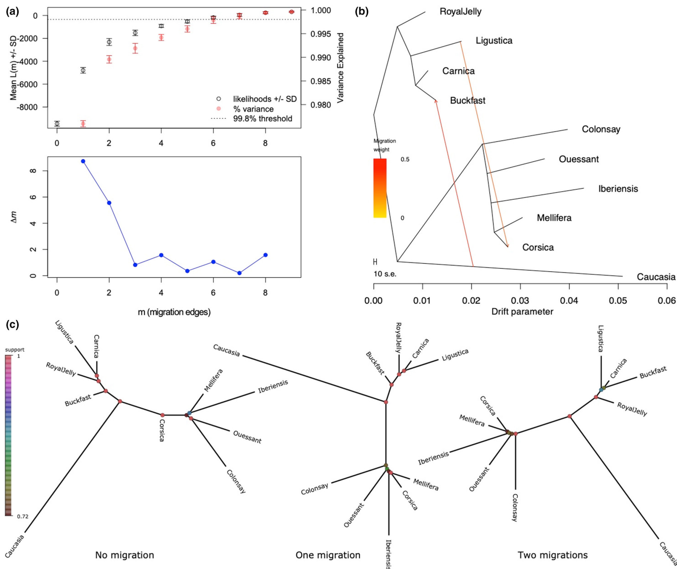
FIGURE 5 Analysis of migrations with TREEMIX. (a) The OptM package was used to determine the optimal number of migrations between populations and backgrounds. The \Delta m values suggest one or two migrations. (b) TREEMIX graph selected amongst the 100 runs showing the two migrations identified. (c) Summaries of 100 trees from TREEMIX, estimated from the 100 runs per migration with DENDROPY. The topologies correspond to the hypothesis of no migration (left), the Corsican population as being of the Apis mellifera mellifera subspecies, with a migration from an A. m. ligustica population (middle) or with an additional migration of A. m. caucasia in the Buckfast population (right). Support for the nodes is indicated by the colour, with values indicated by the scale on the left. Results suggest the original Corsican population is very similar to A. m. mellifera from mainland France
