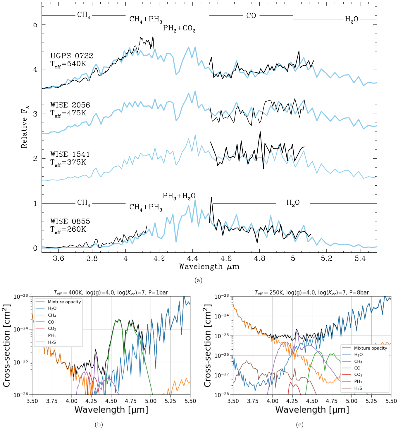
Figure 10. The upper panel (a) shows observations (black line) and the tuned-adiabat model spectra (blue line) from Figures 8 and 9, for 3.5 \leq \lambda \mu\text{m} \leq 5.5 . The lower panels (b)(c) show ATMO 2020 opacity calculations for these wavelengths, for two representative values of T_{\text{eff}} .
