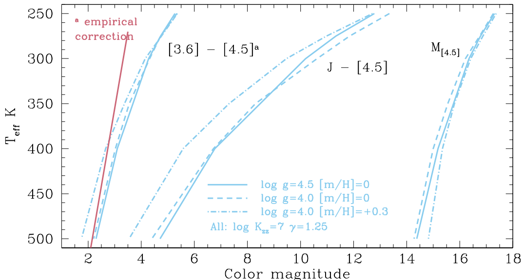
Figure 14. Synthetic colors from the modified-adiabat model grid, see text. Table 4 gives polynomial fits to the solar metallicity relationships shown in the Figure.
