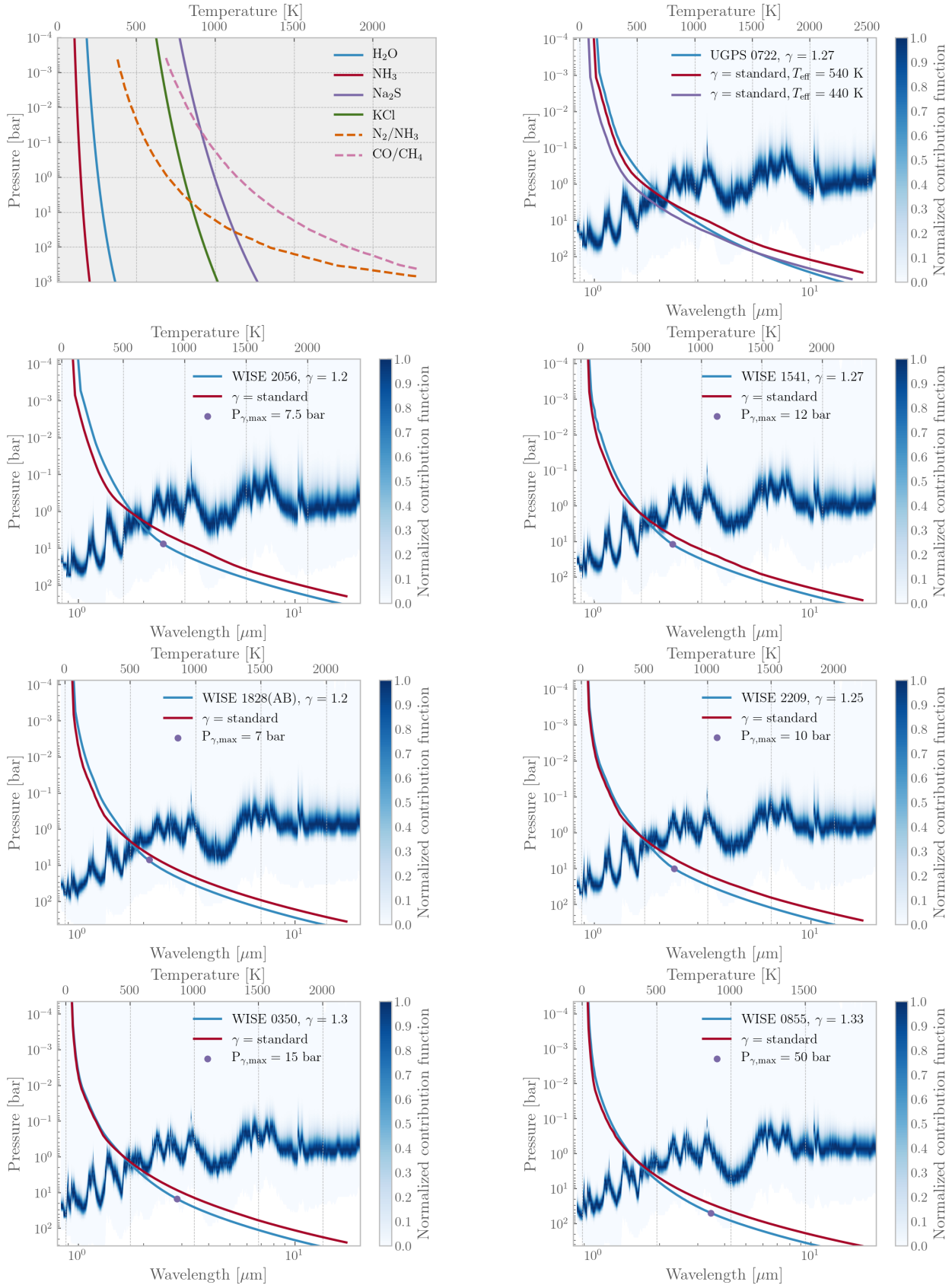
Figure 7. The top left panel shows condensation curves for elements in equilibrium (see text for discussion). The other panels are pressure-temperature profiles (left and upper axes) and flux contribution functions (thick blue line, left and lower axes), for the brown dwarfs in our tuning sample. Blue P - T profiles are tuned to fit the data by reducing the adiabat \gamma at P < P_{\gamma,\text{max}} ; red lines have a standard radiative-convective profile.
