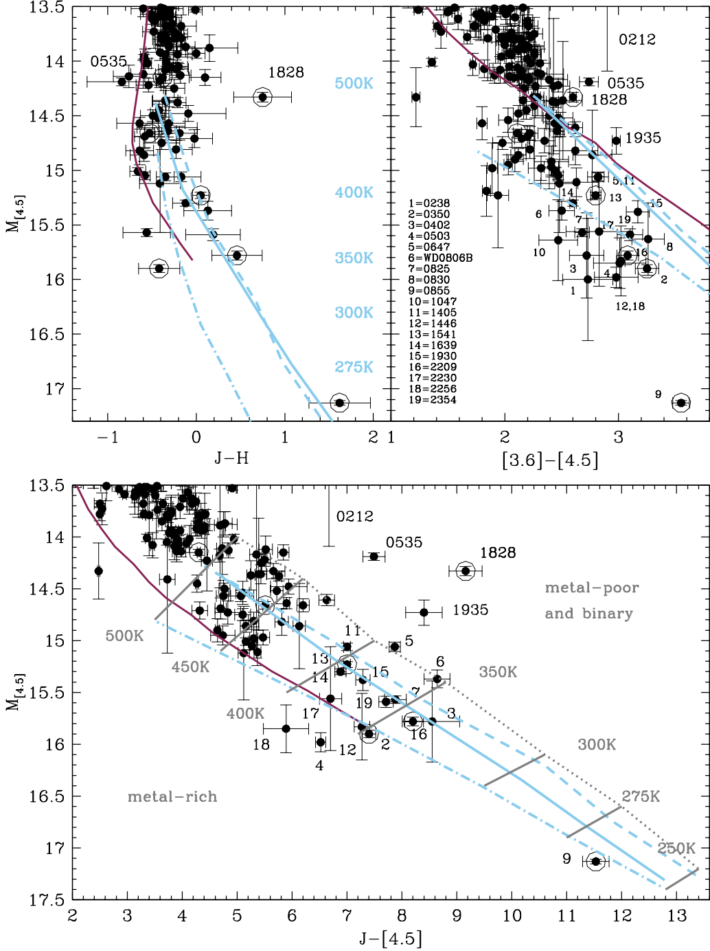
Figure 13. Color-magnitude diagrams for late T and Y dwarfs. Sequences are as in Figure 12. Grey \sim diagonal lines in the bottom panel indicate constant T_{\text{eff}} , as labelled, for metallicities ranging from approximately +0.3 on the left, to -0.5 on the right. The location of the metal-poor envelope edge in the bottom panel is consistent with the low-metallicity Sonora-Bobcat models (Figure 3), and with the observed population. Our SED analysis of J1828 indicates that it is an equal-mass binary with [m/H] \sim -0.5 (Figure 8). J0212, J0535, and J1935 are also likely to be similar-mass binary systems. Notionally single Y dwarfs which are estimated to have T_{\text{eff}} \lesssim 400 K are identified in the legend by the first four digits of the WISE catalog Right Ascension, or their binary name in the case of the white dwarf companion.
