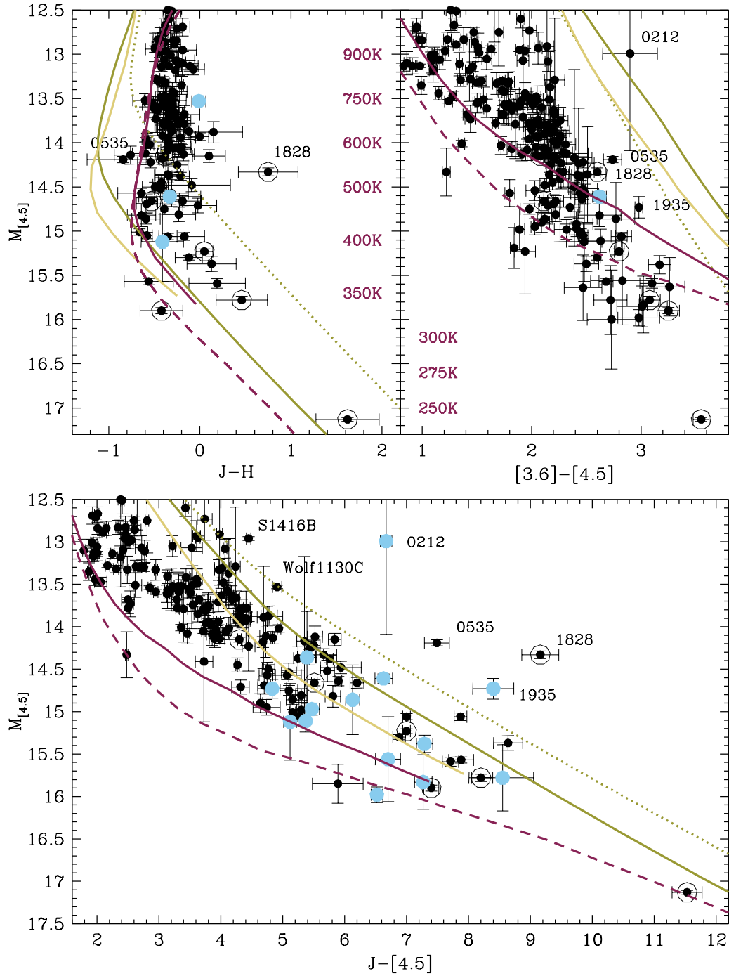
Figure 3. Color-magnitude diagrams for late T and Y dwarfs. Symbols and lines are as in Figure 2. Approximate T_{\text{eff}} values along the top middle axis are from the ATMO 2020 non-equilibrium chemistry models. Over-luminous Y-dwarfs which are possibly unresolved binaries are identified: CWISEP J021243.55+053147.2, WISE J053516.80-750024.9, WISEPA J182831.08+265037.8, and CWISEP J193518.59-154620.3. In the lower panel, the metal-poor T dwarfs S1416B and Wolf 1130C are identified (see also Figure 2).
