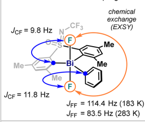
D. ^1\text{H} - ^{19}\text{F} HOESY NMR analysis of 26
