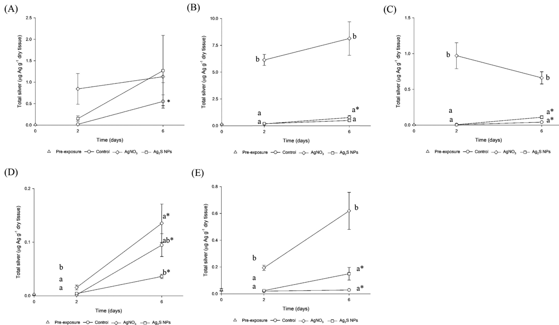
Fig. 3. Total measured silver concentration ( \mu\text{g Ag g}^{-1} ) in dry tissue of rainbow trout ( Oncorhynchus mykiss ) within (A) intestine, (B) liver, (C) gill, (D) muscle and (E) the remaining carcass, at sampling days 0, 2 and 6, in the mesocosm experiment with \text{AgNO}_3 and \text{Ag}_2\text{S NPs} . Data are mean \pm S.E.M ( n = 4-5 ). Different letters indicate statistically significant differences amongst the treatments, within the respective day of sampling (ANOVA, p < 0.05 ). Absence of letters indicates no statistically significant difference in measured silver concentrations amongst the treatments, within the respective day of sampling. Asterisk “*” refers to statistically significant difference in measured silver concentrations by treatment type, with time (day 2 and day 6). Absence of asterisk symbols indicates no statistically significant differences in measured silver concentrations, for each treatment type, with time ( t -test, p > 0.05 ).
