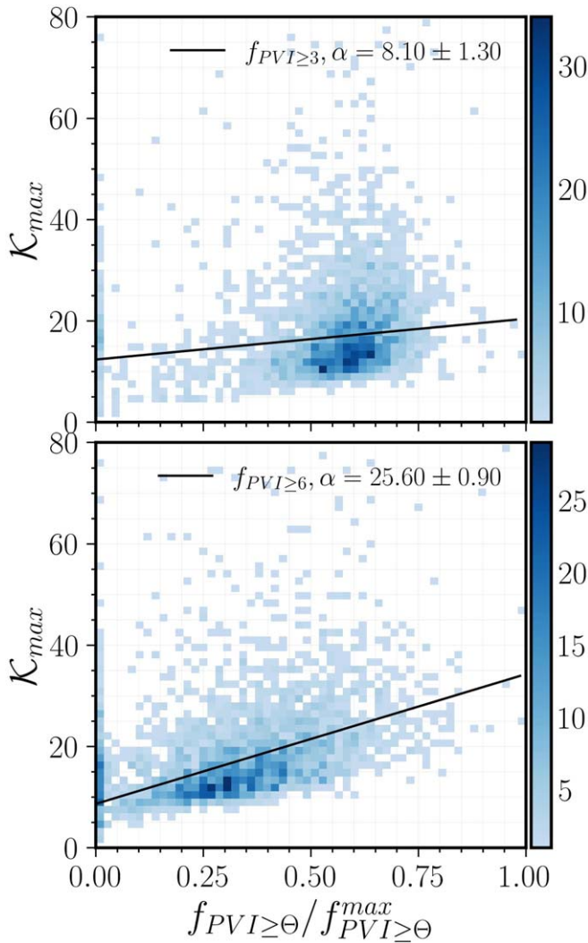
Figure 15. The maximum of SDK, K_{max} , is plotted as a function of the fraction of PVI events that exceed a threshold \theta , f_{PVI \geq \theta} for \theta = 3, 6 , shown in the top and bottom panels, respectively. For a more direct comparison of the two curves, f_{PVI \geq \theta} was normalized to the maximum value f_{PVI \geq \theta}^{max} estimated for the respective threshold.
