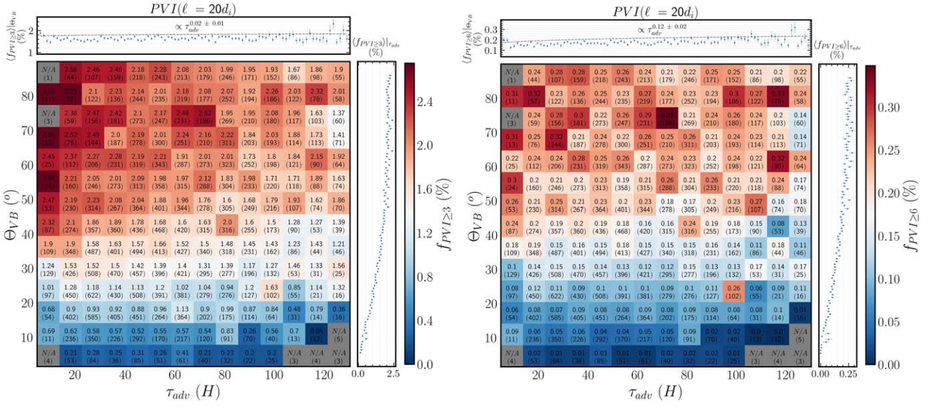
Figure 9. Binned mean of the fraction of data points with PVI values exceeding a given threshold, f_{PVI > \theta} , where \theta = 3 (left panel) and \theta = 6 (right panel), shown as a function of the advection time \tau_{adv} and the angle \Theta_{VB} . The PVI time series was estimated with a lag \ell = 20 d_i . The top subplot shows the averaged fraction of coherent structures over \Theta_{VB} , \langle f_{PVI > \theta} \rangle_{\Theta_{VB}} . Power-law fits are also shown as black dashed lines. Similarly, the right subplot shows the averaged fraction over \tau_{adv} , \langle f_{PVI > \theta} \rangle_{\tau_{adv}} .
