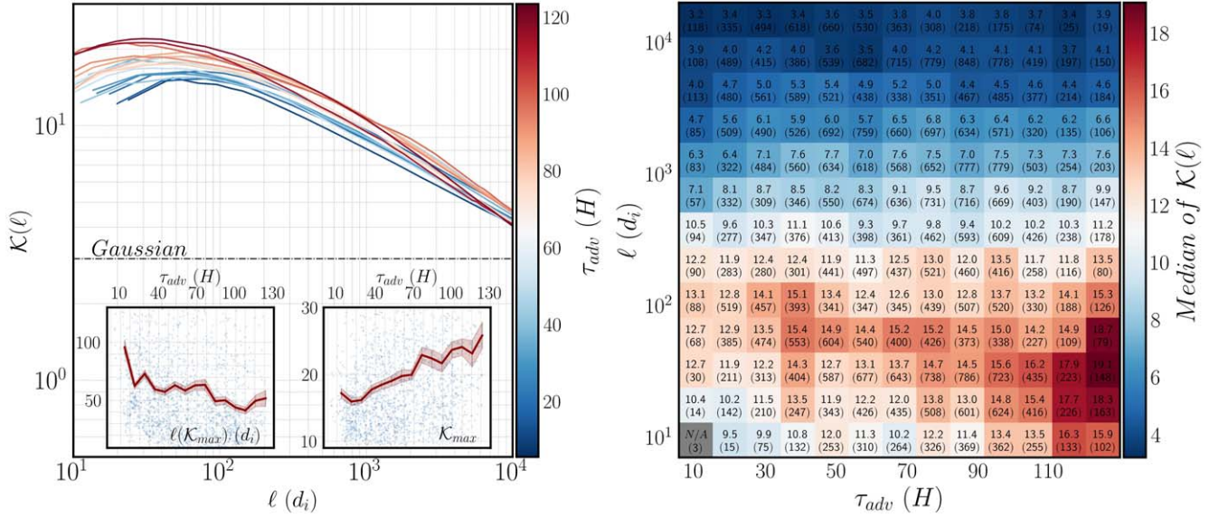
Figure 2. (a) Evolution of SDK with \tau_{\text{adv}} . Each line represents the average of 100 intervals that fall within the same \tau_{\text{adv}} bin. The inset scatter plots show (i) the scale, in units of d_i , at which the kurtosis attains the maximum value; (ii) the maximum kurtosis value estimated for the individual 5H intervals. The binned mean of the two quantities is also shown with a red line. (b) Scale-dependent kurtosis of the magnetic field as a function of the scale in units of the ion inertial length d_i and SW convection time \tau_{\text{adv}} . The numbers indicate the median value of kurtosis within each bin, and the bracketed numbers show the number of events within each bin.
