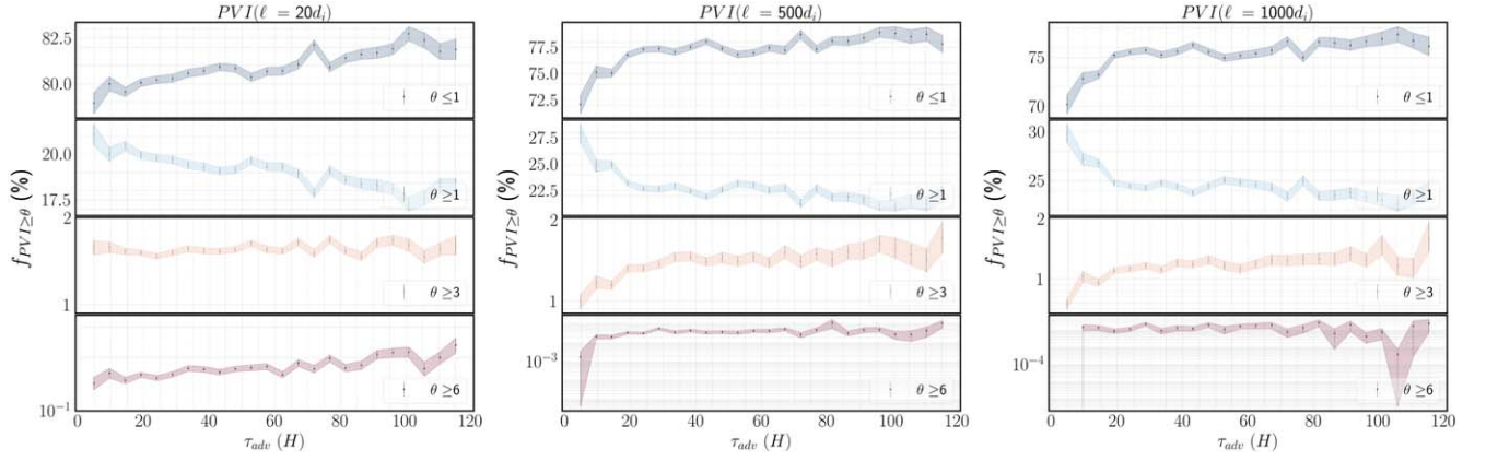
Figure 6. Binned mean of the fraction of data points with PVI values exceeding a given threshold ( f_{PVI \geq \theta} , where \theta = [1, 3, 6] ) shown as a function of the advection time \tau_{adv} ; different thresholds are shown in different colors. Three spatial lags normalized to the ion inertial length d_i are considered: \ell = 20, 500, 1000 d_i .
