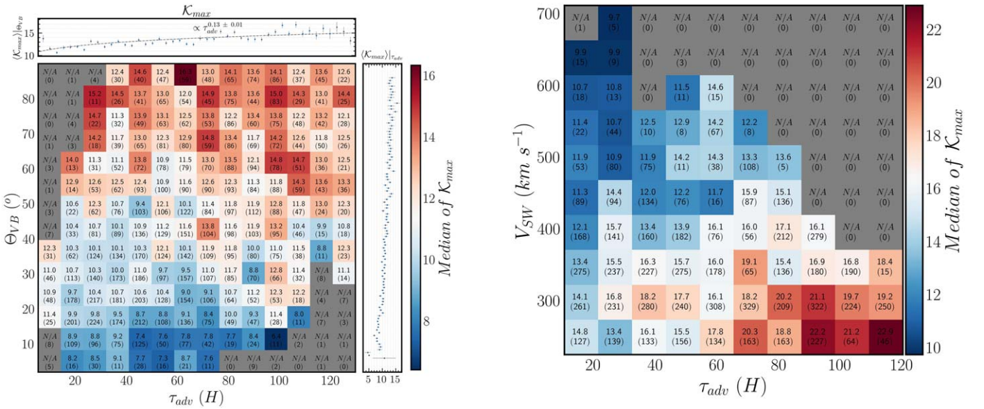
Figure 11. (a) Scale-dependent kurtosis of the magnetic field as a function of the solar wind speed V_{SW} and the SW advection time \tau_{adv} . The numbers indicate the median value of kurtosis within each bin.
