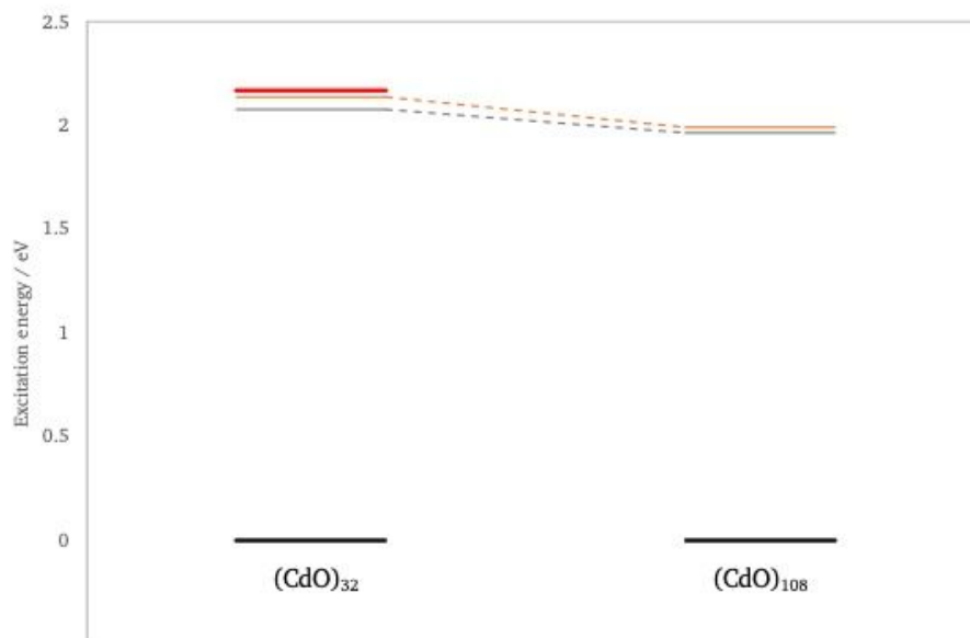
Fig. 8 Change in the predicted optical spectra of (\text{CdO})_{32} with particle size as calculated with evGW(AC)-BSE/def2-SV(P). Red lines T_2 irrep, orange lines T_1 irrep and grey lines a irrep.
