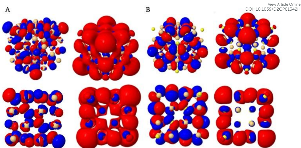
Fig. 5 Highest occupied and lowest unoccupied Kohn-Sham orbitals of (\text{CdO})_{32} (A, left and right, respectively) and (\text{CdS})_{32} (B, left and right, respectively). The top and bottom rows show the same orbitals but from a different perspective. As the calculation were performed using the D_2 instead of the T_d point group, the highest occupied orbital for (\text{CdO})_{32} , a triply degenerate T_1 orbital in T_d , is described as a triplet of orbitals of B_1 , B_2 and B_3 symmetry, where only one of these three is shown here (A, left).
