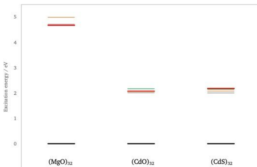
Fig. 4 evGW-BSE/def2-TZVPP predicted optical spectra of (\text{MgO})_{32} , (\text{CdO})_{32} and (\text{CdS})_{32} . Red lines T_2 irrep, orange lines T_1 irrep, green lines e irrep and grey lines a irrep.
