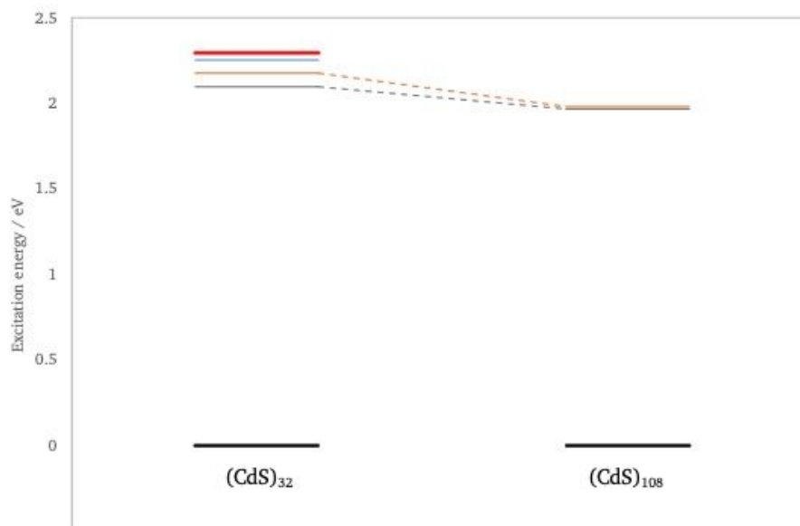
Fig. 9 Change in the predicted optical spectra of (\text{CdS})_{32} with particle size as calculated with \text{evGW(AC)-BSE/def2-SV(P)} . Red lines T_2 irrep, orange lines T_1 irrep, blue lines e irrep and grey lines a irrep.
