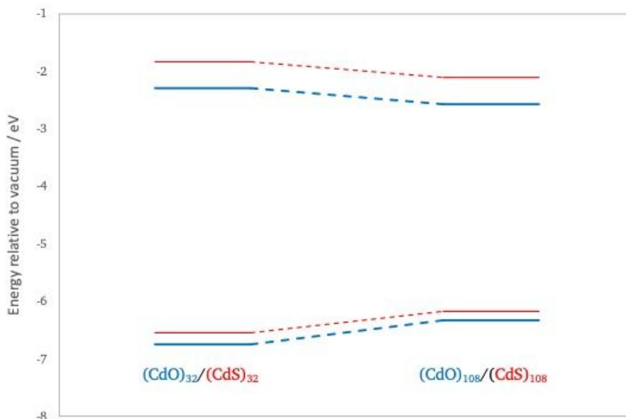
Fig. 7 Change in the highest occupied and lowest unoccupied quasiparticle states with particle size as calculated with evGW(AC)/def2-SV(P) , showing the two highest occupied and two lowest unoccupied quasiparticle states
