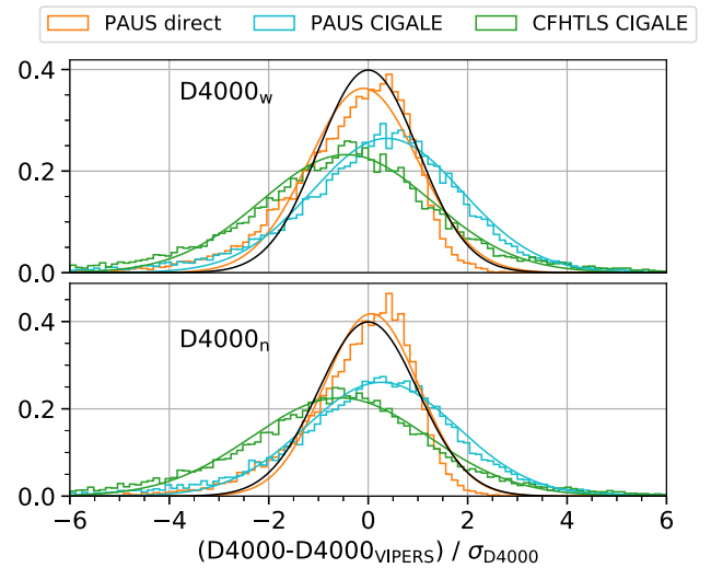
Figure 8. Distribution of the difference between D4000 estimations and VIPERS D4000 values, divided by the estimated error. All distributions are accompanied of their respective Gaussian fit; the solid black line shows a reference Gaussian with \mu = 0 and \sigma = 1 . Upper panel: D4000_w . Lower panel: D4000_n .
