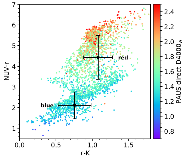
Figure 13. NUVrK colour diagram for the bright sample, colour-coded with the PAUS direct D4000_w (with colour scale limited by the outlier cuts defined for VIPERS D4000 ). The average positions of the red/blue galaxies from our fiducial classification are also displayed, with their errorbars being their standard deviations.
