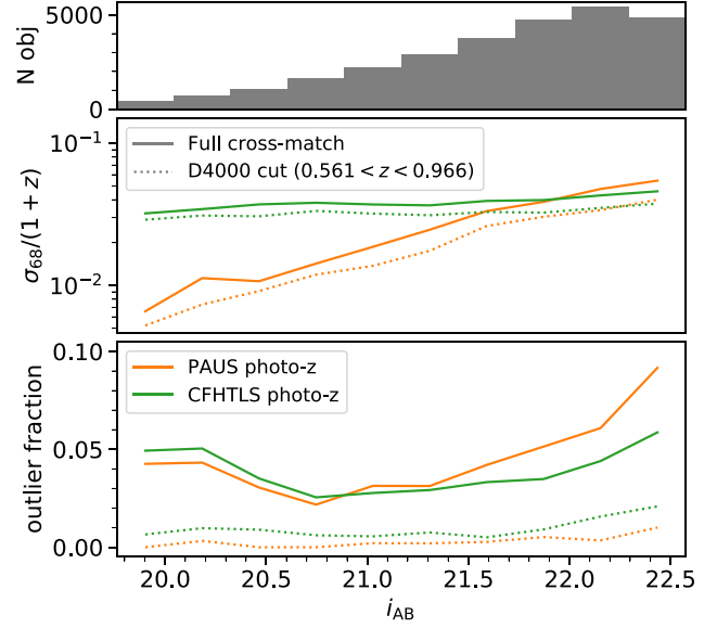
Figure A2. \sigma_{68}/(1+z) (middle panel) and outlier fraction (lower panel) for the PAUS photo- z (orange lines) and CFHTLS photo- z (green lines), in magnitude bins. The solid line represents the full cross-match, dotted line the redshift cut for D4000 measurement. Upper panel displays the magnitude histogram.
