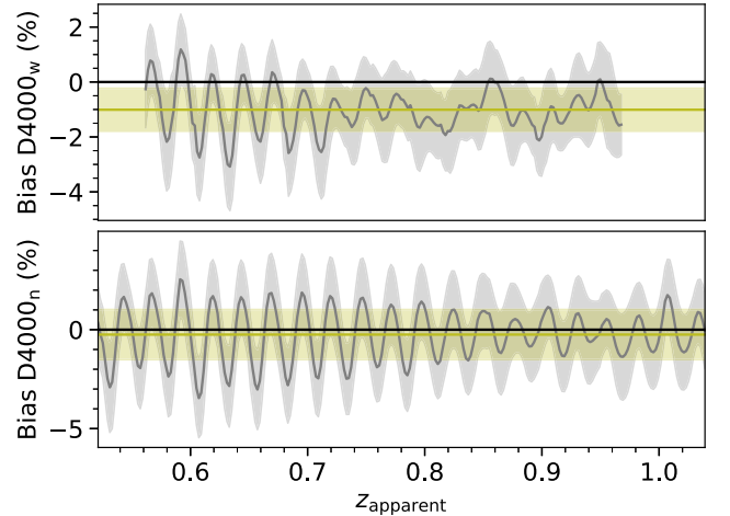
Figure 5. Bias versus z_{\text{apparent}} for the sPAUS D4000 w (upper panel) and sPAUS D4000 n (lower panel). The grey line and shaded area represent the mean bias and its \sigma for each z_{\text{apparent}} , while the yellow line and its shaded area are the mean bias and \sigma for the whole z_{\text{apparent}} range.
