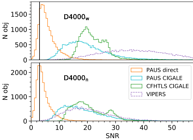
Figure 7. SNR distribution for PAUS direct, PAUS CIGALE, CFHTLS CIGALE, and VIPERS spectroscopy. The black vertical line displays the detection threshold of \text{SNR} > 3 . Upper panel: D4000_w . Lower panel: D4000_n .
