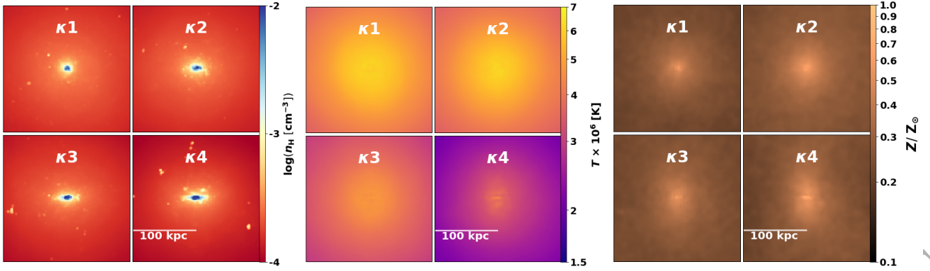
Figure 9. Physical property stacked maps of the hot gas within 200 \times 200 kpc panels: hydrogen number density (left panels), temperature (middle panels), and metallicity (right panels). Each panel set shows the 4 subsamples: \kappa 1 (top left), \kappa 2 (top right), \kappa 3 (bottom left), and \kappa 4 (bottom right). Higher \kappa galaxies have more elliptical extended gas CGMs beyond the disc, which are slightly lower density than spheroids. The temperature panels show cooler gas around discs than spheroids, indicative of discs living in lower mass haloes. Bipolar metal-enriched outflows are apparent in disc galaxies.
