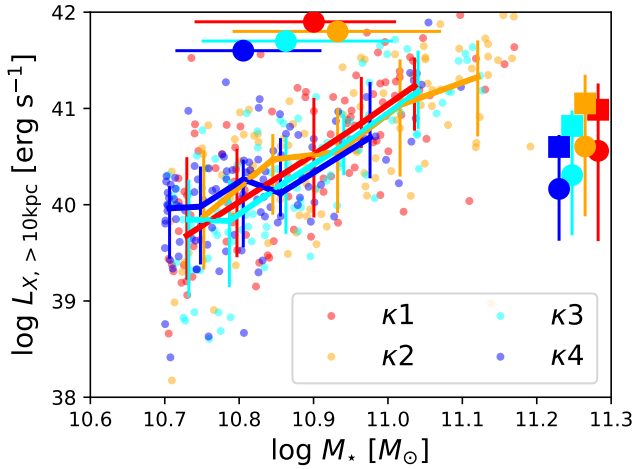
Figure 11. Extended ( > 10 kpc) X-ray emission as a function of stellar mass divided into our 4 morphological samples with points showing individual galaxies and solid lines showing medians. Lines are adaptive bins that divide the 107-galaxy samples into 5 equally sized M_{*} bins with vertical error bars showing the 1-\sigma spread. There is no obvious trend for L_{X, > 10\text{kpc}} on morphology at fixed M_{*} . Large circles and error bars on the top and to the right show the median and 1-\sigma dispersion for each distribution. Brighter spheroidal haloes have a higher distribution of M_{*} than disc haloes. Large squares indicate the mean L_{X, > 10\text{kpc}} .
