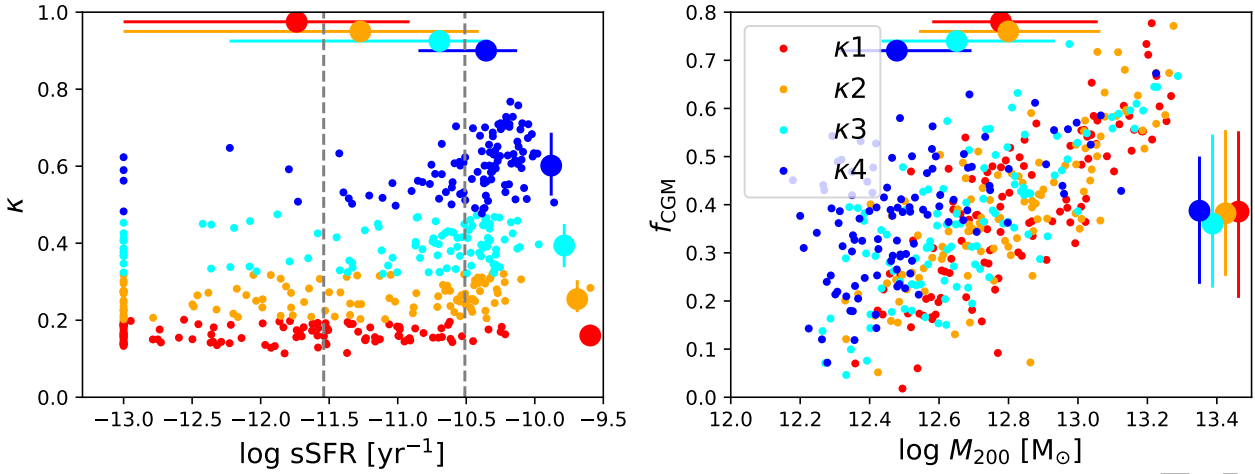
Figure 1. Our EAGLE galaxy subsamples, coloured from red to blue for \kappa 1 (spheroids) to \kappa 4 (discs). The left panel plots two galaxy characteristics for the M_{\star} = 10^{10.7-11.2} M_{\odot} samples. sSFR correlates with \kappa . \text{sSFR} \leq 10^{-13} \text{ yr}^{-1} are plotted as having 10^{-13} \text{ yr}^{-1} . The right panel plots two halo-wide characteristics, virial mass versus f_{\text{CGM}} , which is the fractional gas content of the CGM relative to its expected total baryon content. Large circles and error bars on the top and to the right show the median and 1-\sigma dispersion for each distribution. The dashed lines in the right panel indicate the low-sSFR (left of left line) and high-sSFR (right of right line) samples of O20.
