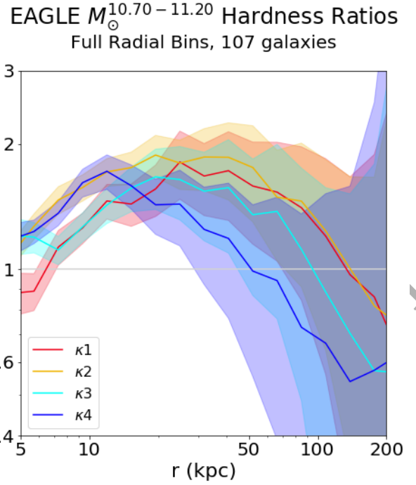
Figure 5. Hardness ratios (ratio of highest-energy stacks to lowest-energy stacks) of the galaxy subsamples. The Poisson errors here show how difficult it is to distinguish hardness ratios between samples, although the \kappa4 sample does indicate hotter gas in the center, while the spheroid samples have hotter gas in their exteriors than discs.
