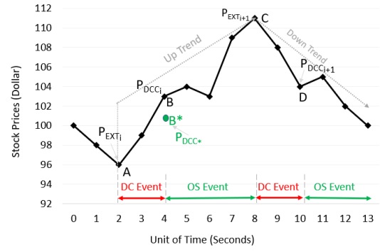
Fig. 1. Transformation of 14 unit of physical time data into event-based series by DC. There are two DC event confirmation at time 4 and 10. Concluded up trend takes place between the two extreme points, A and C, which are confirmed retrospectively at their subsequent confirmation points, B and D.
