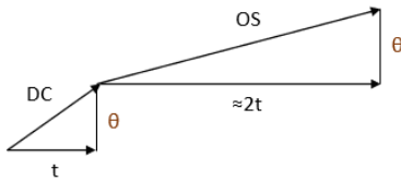
Fig. 2. Two scaling laws from [6], which are implemented in our strategies, that shows (a) price changes in DC and followed OS is approximately same and equals to threshold, (b) if DC event takes t physical time, its subsequent OS takes approximately 2t .
