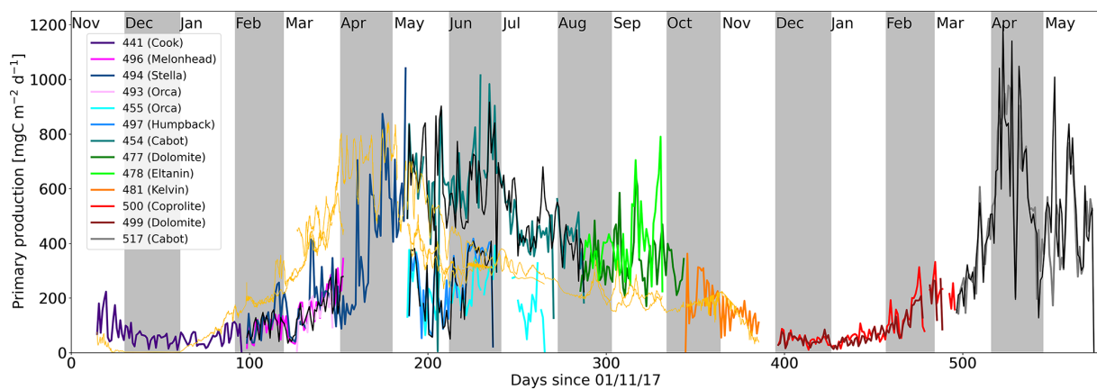
Figure 9. Daily integrated net primary production rate estimates from all gliders deployed in the AlterEco programme (see Table 1). Coloured traces represent each glider mission (matching those used in Fig. 1) and show the net primary production estimates derived from the SEO-based PAR method. Where in situ PAR sensors were available, a corresponding black trace for that glider mission is also shown. The thin orange trace shows the net primary production extracted from v4.2 of the ESA Ocean Colour Climate Change Initiative (OC-CCI) NPP product for each glider where available.
