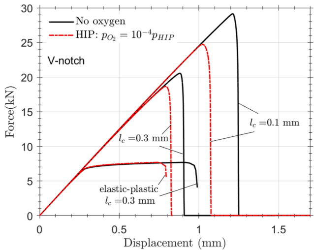
Fig. 17. Oxygen influence on V-notch fracture for a non-inert atmosphere during HIP.
