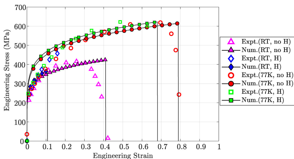
Fig. 12 – Role of temperature on the failure of polycrystalline Ni samples: engineering stress-strain curves for both H-charged and non-charged samples pulled to failure at 77K and at ambient temperature (298 K).
