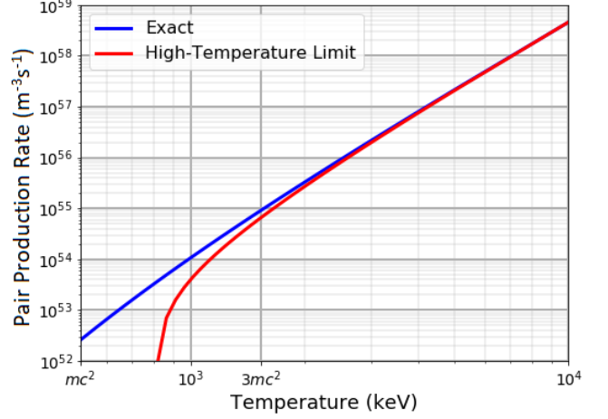
Figure 1: Approximation of thermal Breit-Wheeler pair creation rate plotting against numerical calculation, with n, l in equation 1 summed from 1 to 20, at which there is numerical convergence to precision visible on the graph. The approximation is seen to rapidly approach the exact result from below for k_B T > 3mc^2 .
