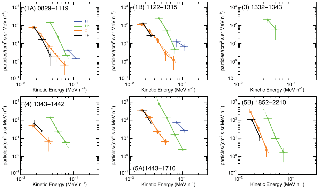
Figure 4. Differential energy spectra for H, He, O, and Fe in six different time intervals associated with the HCS crossing (see Figure 1). Dashed lines represent power-law fits to the He (green), O (orange), and Fe (black) spectra, with the power-law spectral indices provided in Table 1.
