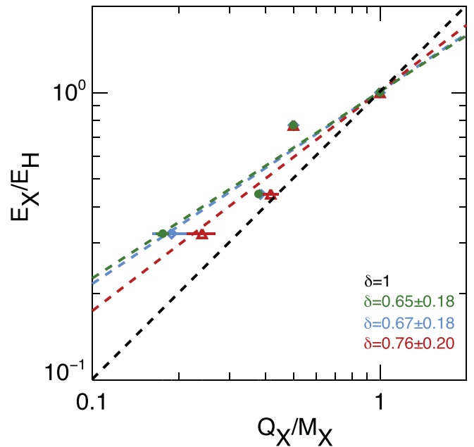
Figure 6. Maximum observed energy E_X vs. ion charge-to-mass ratio for that species. O and Fe ionization states are assumed to be event-averaged charges states measured in the solar wind (green), impulsive (red), and gradual (blue) SEPs. Colored dashed lines represent the corresponding fits to E_X/E_H \propto (Q_X/M_X)^\delta ; the dashed black line represents E_X/E_H \propto (Q_X/M_X) , i.e., \delta = 1 .
