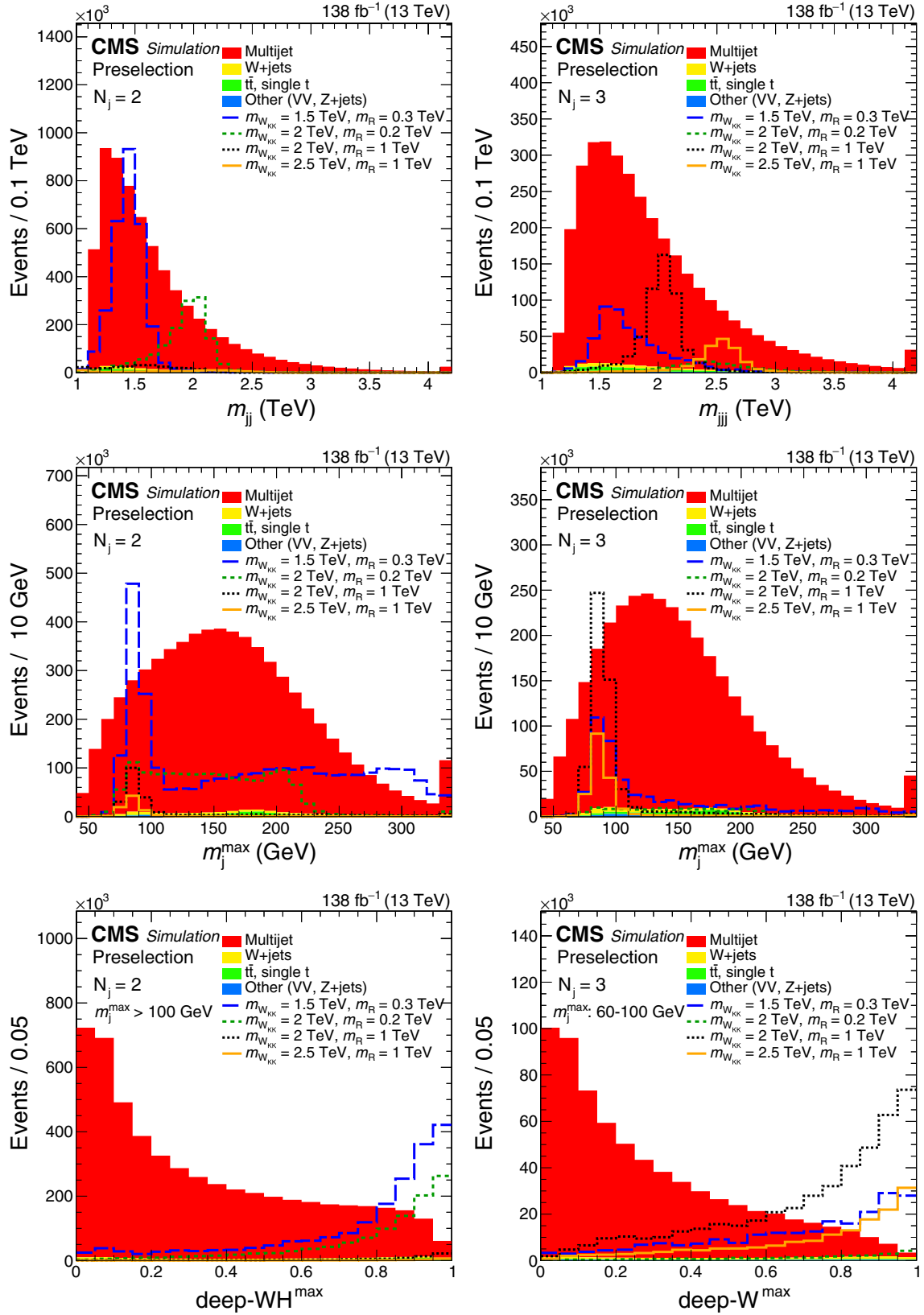
FIG. 2. Variables discriminating between signal and background in simulation. Left column, upper to lower rows: the distributions of m_{jj} , m_j^{\text{max}} , and \text{deep-WH} (for highest mass jet with m_j^{\text{max}} > 100 \text{ GeV} ) for preselected events with N_j = 2 . Right column, upper to lower rows: the distributions of m_{jj} , m_j^{\text{max}} , and \text{deep-W} (for highest mass jet with 60 < m_j^{\text{max}} < 100 \text{ GeV} ) for preselected events with N_j = 3 . The signal processes are scaled to 500 times their theoretical cross sections for visibility.
