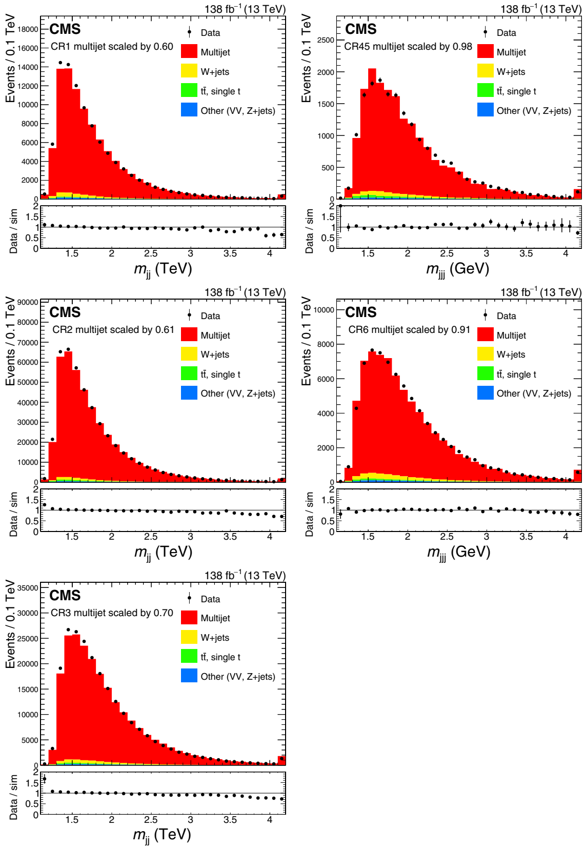
FIG. 8. Invariant mass distributions of the reconstructed triboson systems for control regions in data (black markers) and simulated events (histograms). The m_{\text{triboson}} distributions for CR1, CR2, CR3 are presented in the left column, upper to lower rows, respectively; the m_{\text{triboson}} distributions for control regions CR45 and CR6 are presented in the right column, upper and middle rows, respectively. The simulation is corrected by SFs, and the QCD multijet background is scaled to the data yields.
