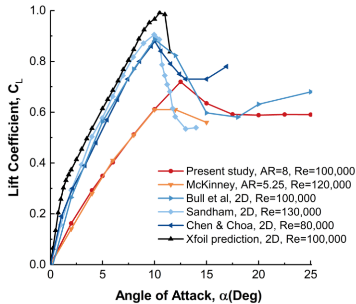
Figure 2: Time-averaged lift coefficient in freestream and comparison with literature.
