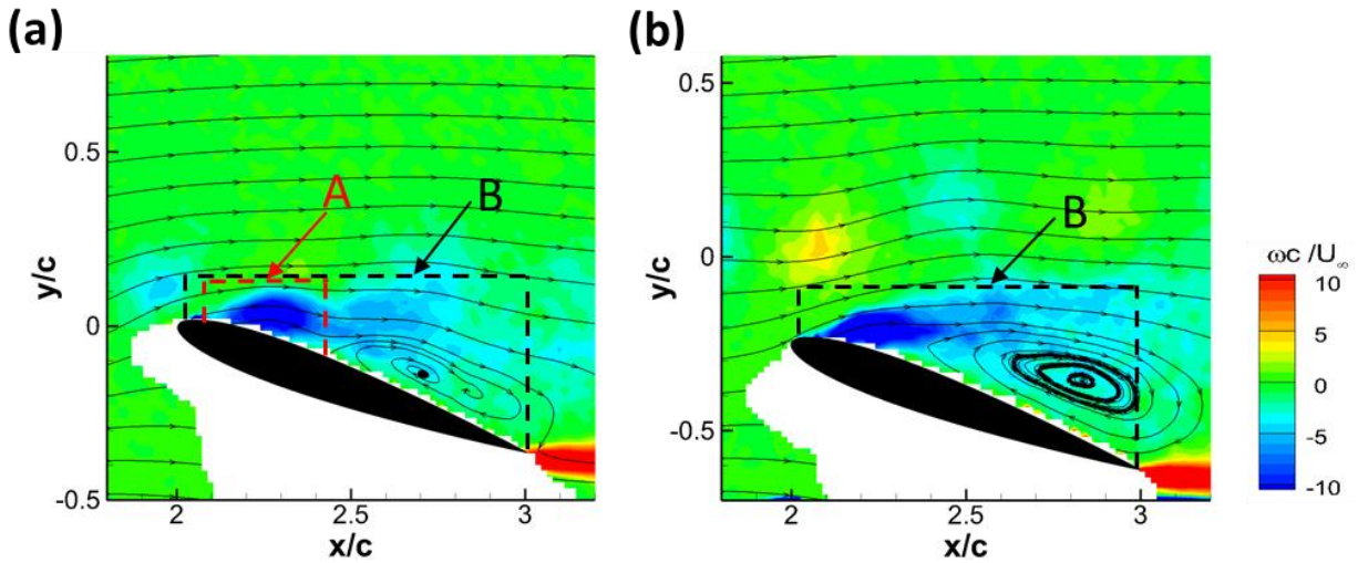
Figure 11: Illustration of the two control volumes for circulation computation, \alpha=20^\circ , H/c=0.2 , at (a) y_{LE}/c = 0 , (b) at y_{LE}/c = \text{optimal location} .
