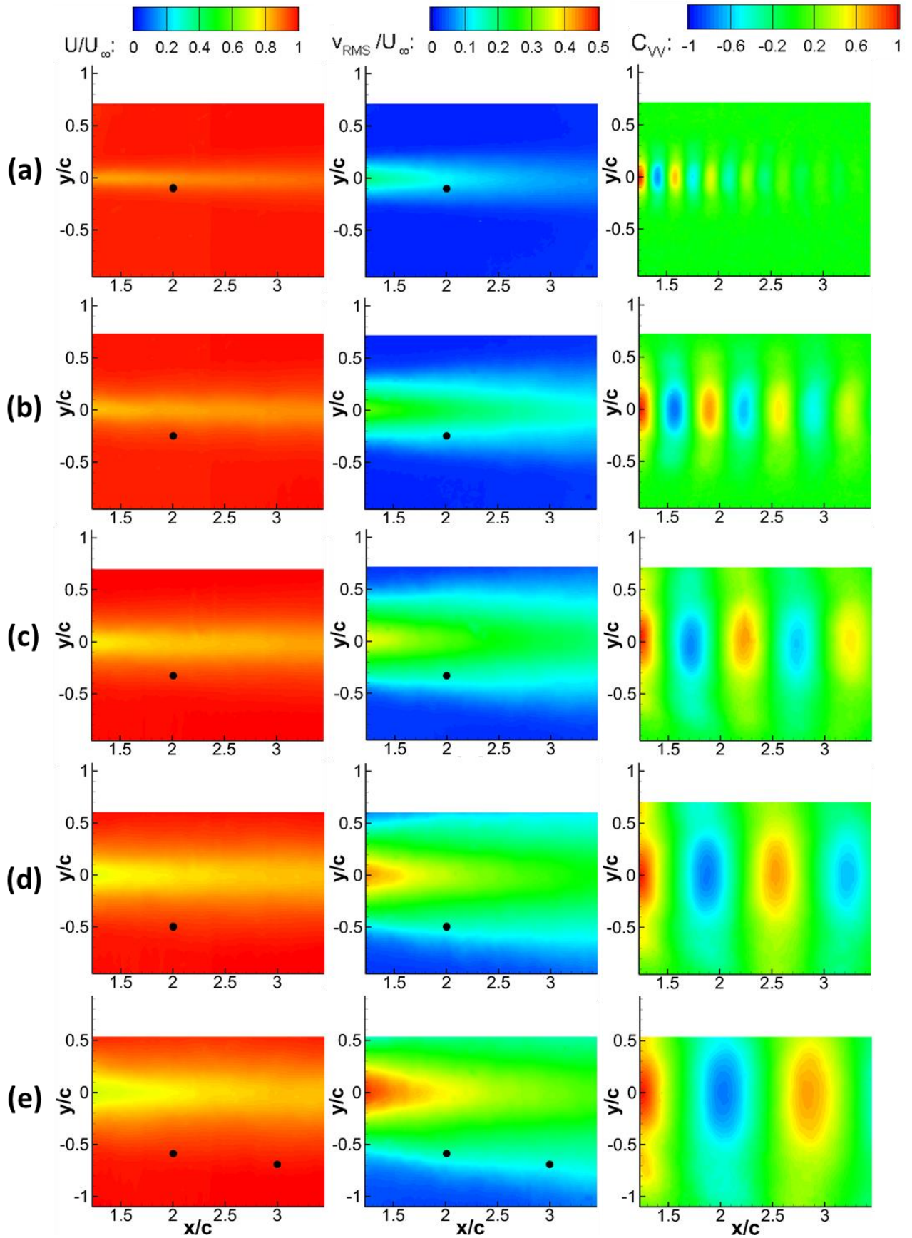
Figure 4: Time-averaged streamwise velocity (left), rms of cross-stream velocity (middle), and cross-correlation of cross-stream velocity (right) for (a) H/c=0.1 , (b) H/c=0.2 , (c) H/c=0.3 , (d) H/c=0.4 , (e) H/c=0.5 . Black dots show the optimal locations.
