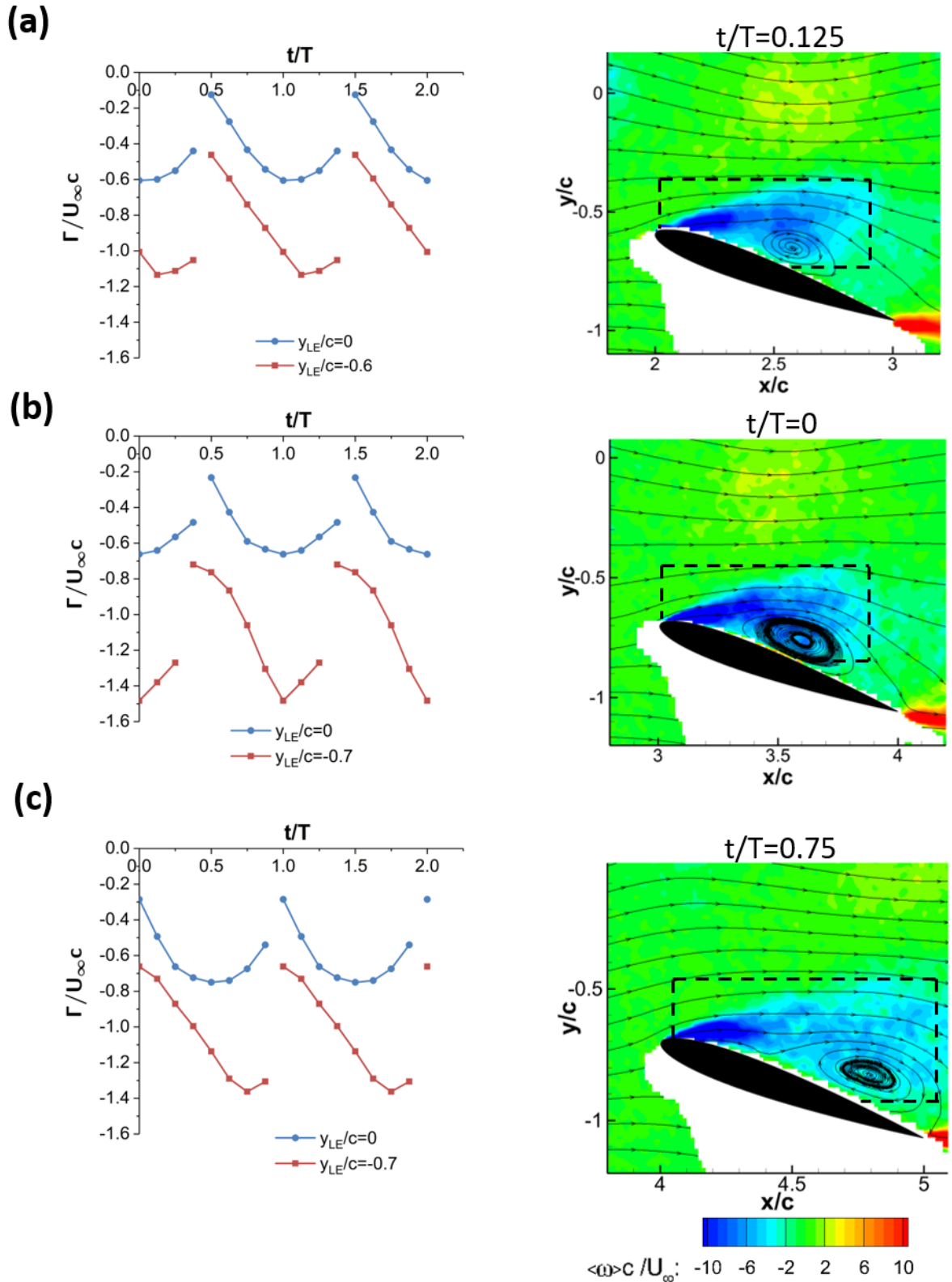
Figure 15: Time history of normalised LEV circulation (left column) and the phase-averaged vorticity contour at the instance with maximum LEV circulation (right column) for \alpha=20^\circ , H/c=0.5 , (a) x_{LE}/c=2.0 , (b) x_{LE}/c=3.0 , (c) x_{LE}/c=4.0 .
