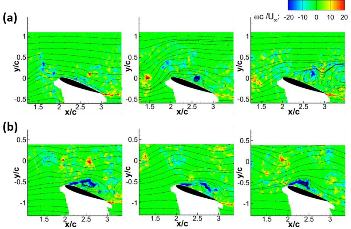
Figure 8: Instantaneous vorticity contours for \alpha=20^\circ , x_{LE}/c = 2.0 , H/c=0.5 , (a) y_{LE}/c = 0 , (b) y_{LE}/c = -0.6 .
