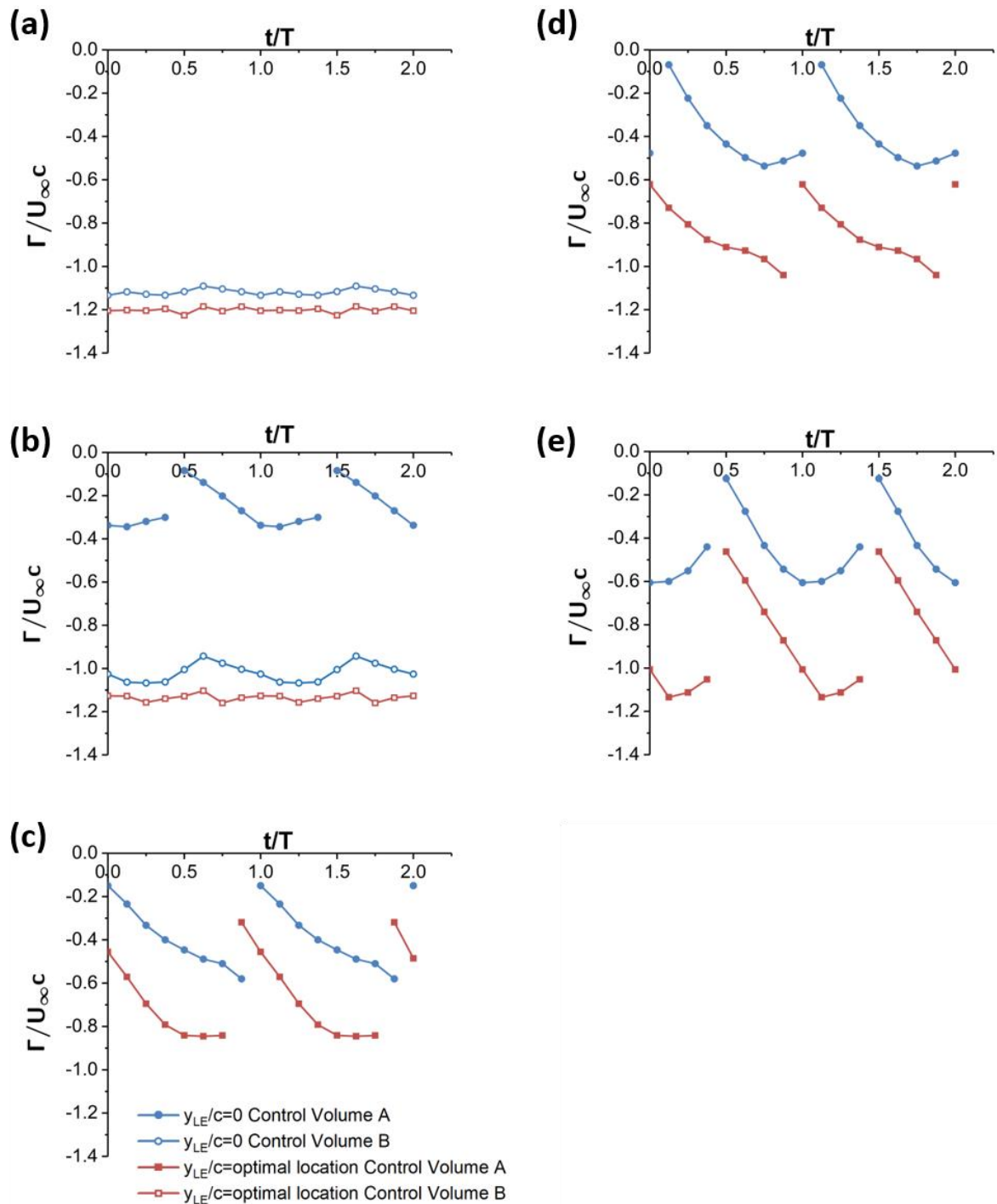
Figure 12: Time history of normalised LEV circulation for \alpha=20^\circ , x_{LE}/c=2.0 , (a) H/c=0.1 , (b) H/c=0.2 , (c) H/c=0.3 , (d) H/c=0.4 , (e) H/c=0.5 .
