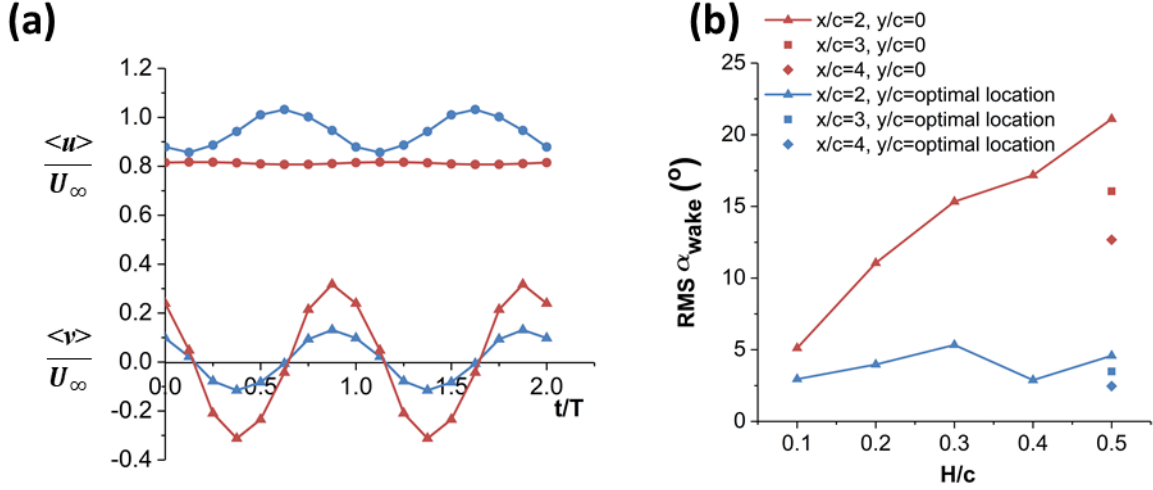
Figure 6: (a) Normalised \langle u \rangle and \langle v \rangle velocity components at wake centreline (red symbols and lines) and optimal location (blue symbols and lines), for x/c = 2.0 and H/c=0.3 ; (b) rms of wake angle as a function of wake generator thickness.
