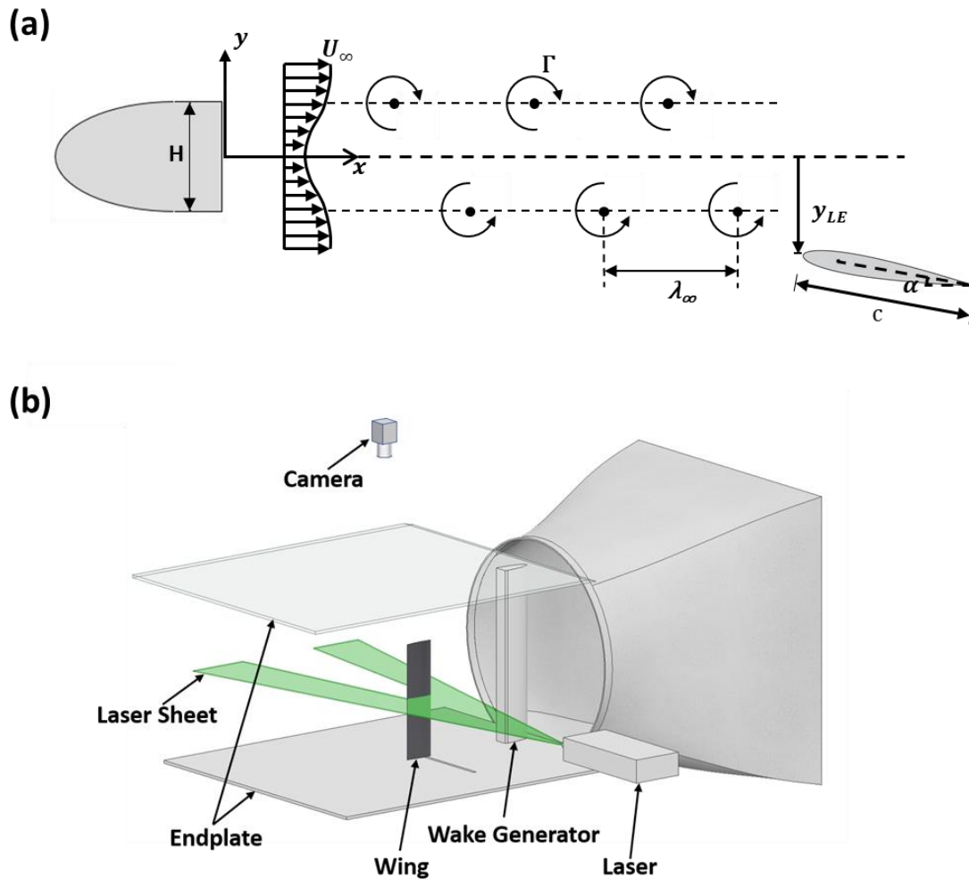
Figure 1: (a) Schematic of the wing in the wakes of bluff bodies; (b) schematic of the experimental setup and the PIV measurements.
