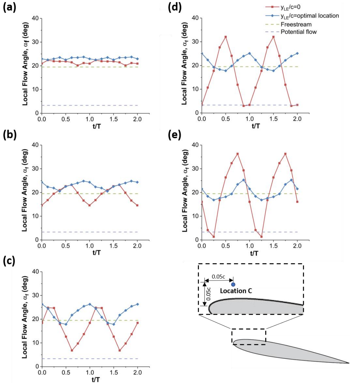
Figure 13: Local flow angle sampled at 0.05c above and downstream of leading-edge for \alpha=20^\circ , x_{LE}/c = 2.0 , at the wake centreline and optimal location, (a) H/c=0.1 , (b) H/c=0.2 , (c) H/c=0.3 , (d) H/c=0.4 , (e) H/c=0.5 .
