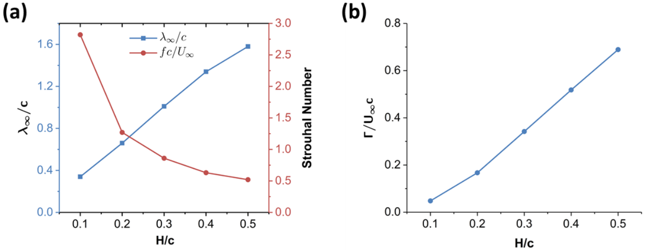
Figure 5: (a) Normalised wavelength and Strouhal number based on chord length, (b) normalised circulation of the wakes as a function of the ratio of the thickness of the wake generator to chord length.
