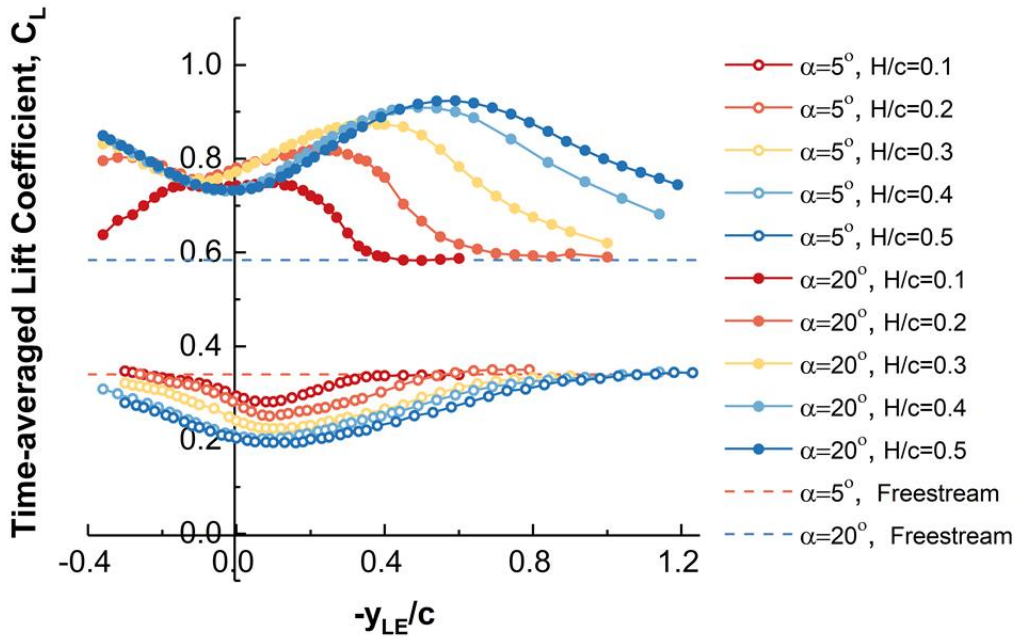
Figure 3: Time-averaged lift coefficient as a function of offset distance at x_{LE}/c = 2.0 .
