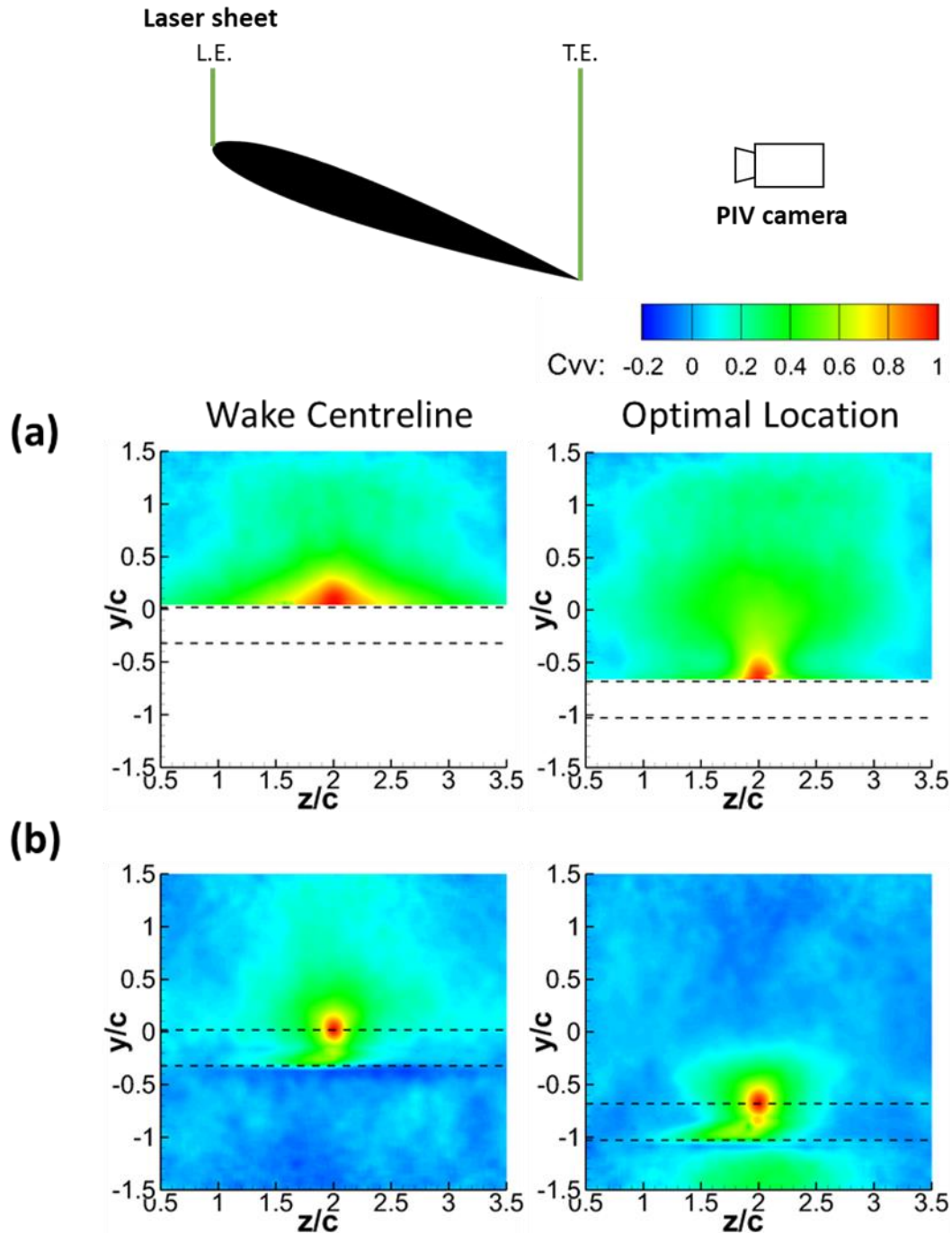
Figure 16: Cross-correlation of cross-stream velocity when the wing was placed at wake centreline and optimal location, \alpha=20^\circ , x_{LE}/c=3.0 , at (a) leading-edge, and (b) trailing-edge.
