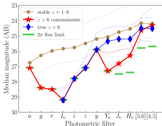
Fig. 4: Median magnitudes of our simulated sources in the Euclid , Rubin, and Spitzer filters. Light brown circles represent stable intermediate- z galaxies, red stars z > 6 contaminants, and blue diamonds true z > 6 galaxies. For each population, the dotted lines indicate the 16 th and 84 th percentiles. For each band, the 2\sigma flux limit is shown with a green bar. The selection of intermediate- z , contaminants, and z > 6 galaxies is based on Euclid +Rubin+ Spitzer data. The median magnitudes for z > 6 galaxies in the Rubin u, g, r bands are equal to -99 (no intrinsic flux) and therefore omitted from this figure.
