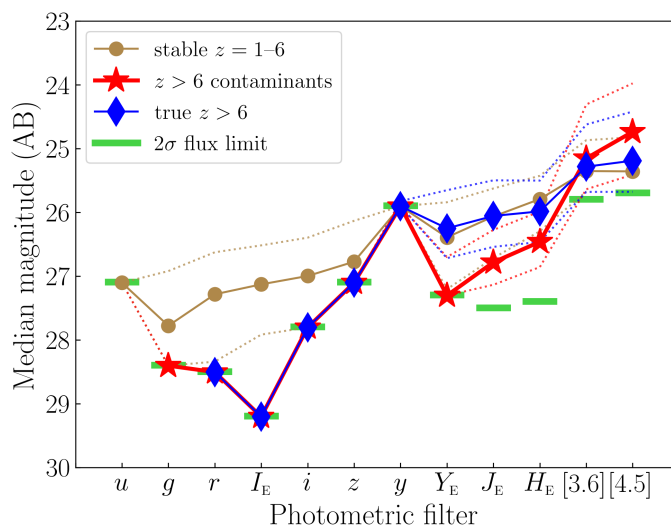
Fig. 14: Median simulated magnitudes of the faint mock sample in the Euclid , Rubin, and Spitzer filters. Light brown circles represent stable intermediate- z galaxies, red stars z > 6 contaminants, and blue diamonds true z > 6 galaxies. For each population, the dotted lines indicate the 16 th and 84 th percentiles. The 2\sigma flux limits are shown with green bars. The selection of intermediate- z , contaminants, and z > 6 galaxies from the faint mock sample is based on Euclid +Rubin+ Spitzer data. The median magnitudes for z > 6 galaxies in the Rubin u and g bands and for contaminants in the Rubin u band are equal to -99 (no intrinsic flux) and therefore omitted from this figure.
