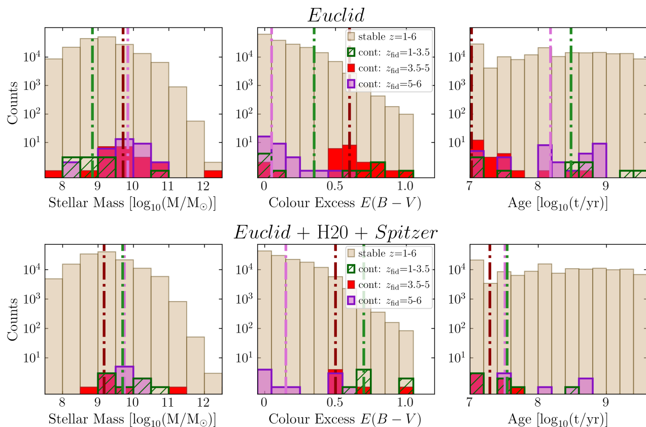
Fig. 9: Fiducial COSMOS photometry-derived stellar mass, colour excess, and age distributions of the stable intermediate- z galaxies (in light brown) and the z > 6 contaminants. The latter are divided into three samples: contaminants with fiducial z = 1-3.5 (in hatched green), contaminants with fiducial z = 3.5-5 (in red) and contaminants with fiducial z = 5-6 (in purple). The median of each distribution is indicated with a vertical line in a corresponding colour. The upper panels show contaminants identified from Euclid data alone, and the lower panels show contaminants identified from Euclid +H20+ Spitzer data.
