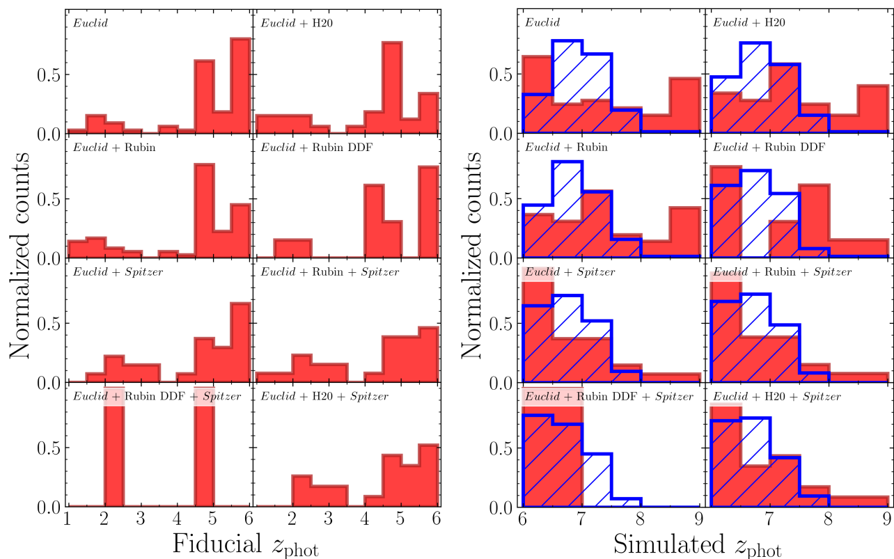
Fig. 7: Photometric redshifts distributions of the intermediate- z interlopers. (Left panel) Normalised fiducial redshift distribution of the z > 6 contaminants in each scenario of Euclid (+ancillary) photometry. (Right panel) Normalised Euclid (+ancillary) photometry-derived redshift distributions of the true z > 6 galaxies (in hatched blue) and z > 6 contaminants (in red).
