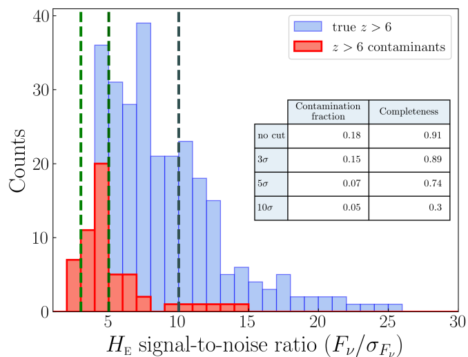
Fig. 6: Histogram of the H_E -band S/N. Contaminants and true z > 6 galaxies as identified from Euclid data alone are displayed in red and blue graphs, respectively. The vertical dashed lines indicate the 3\sigma , 5\sigma , and 10\sigma detection cutoffs. The contamination fraction and completeness computed for the three cuts are indicated in the table.
