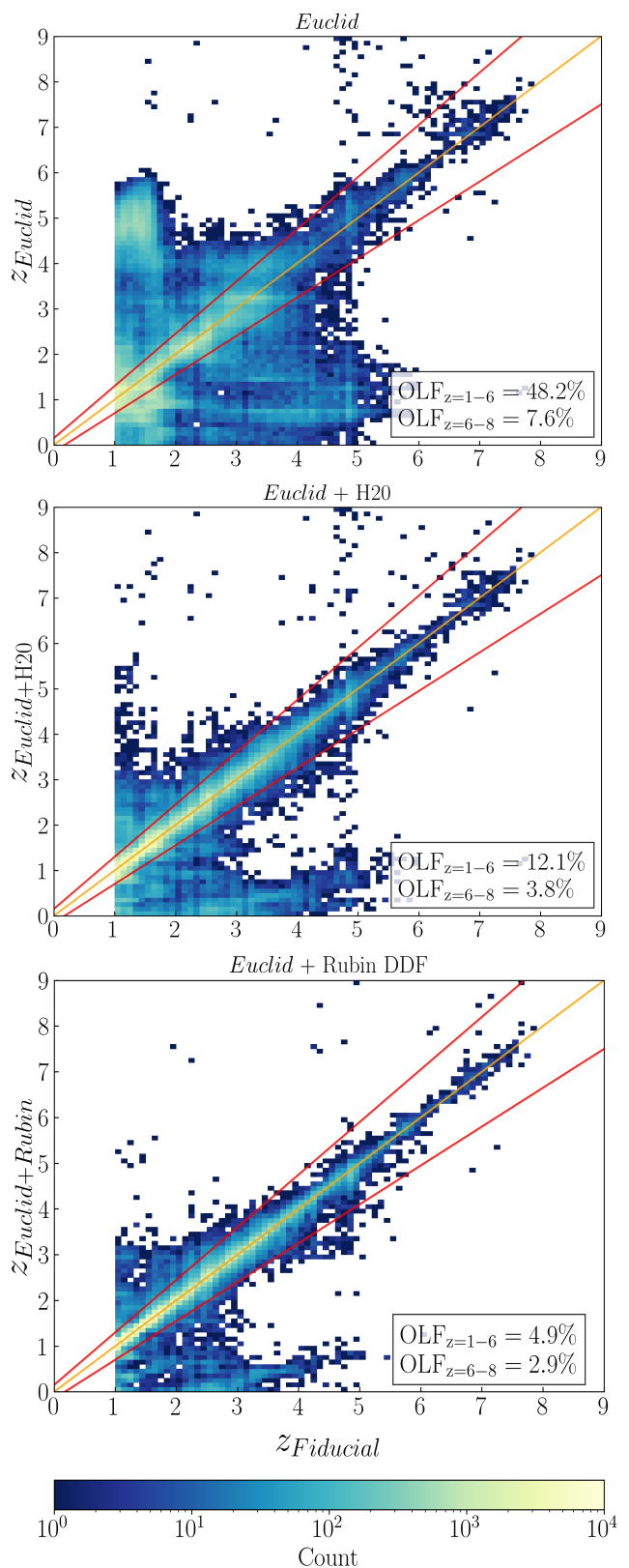
Fig. 3: Comparison of the fiducial photometric redshift to the photometric redshift obtained from three combinations of Euclid and ancillary photometry. In each panel, the catastrophic outlier fractions (OLFs) are reported for two fiducial redshift bins, z = 1-6 and z = 6-8 . The OLF represents the fraction of sources with |z_{\text{sim}} - z_{\text{fid}}| / (1 + z_{\text{fid}}) > 0.15 . The outlier identification boundaries are indicated with solid red lines. The data points are presented as 2D histograms with bin size \Delta z = 0.1 . The colour bar corresponds to the number of galaxies in each bin and is the same for all panels. The solid orange line is the identity curve. Data outside the two solid red lines is identified as catastrophic outliers.
