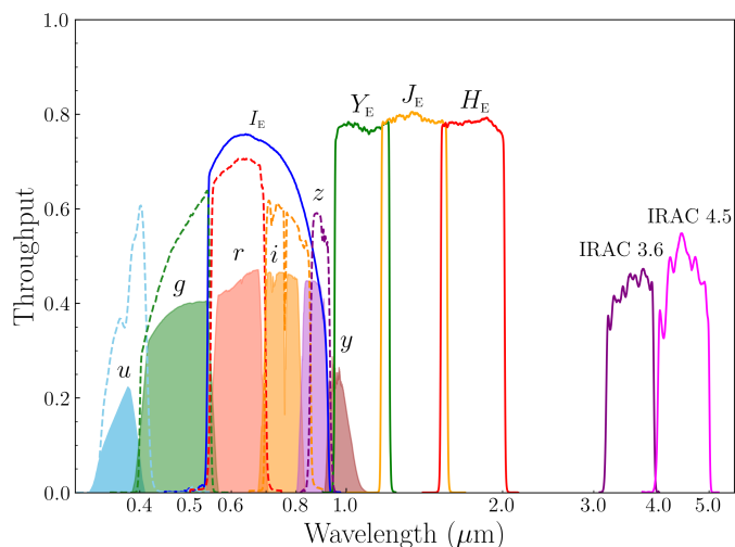
Fig. 2: Transmission curves of the Euclid I_E , Y_E , J_E , and H_E filters, the Rubin u , g , r , i , z , and y filters (filled-in, solid curves), the CFHT u and Subaru HSC g, r, i , and z filters (open, dashed curves), and the Spitzer IRAC 3.6 and 4.5 \mu\text{m} filters.
