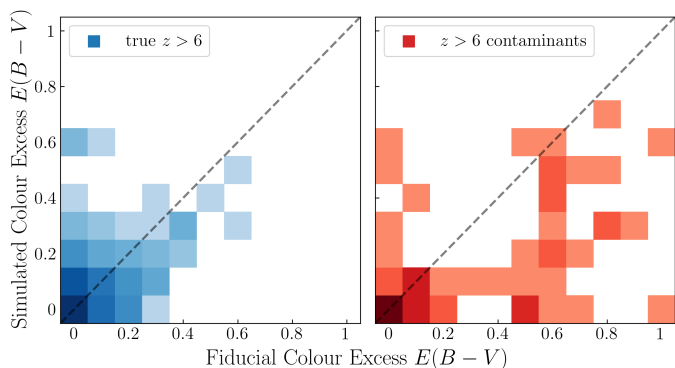
Fig. 12: Fiducial colour excess versus Euclid photometry-derived colour excess for true z > 6 galaxies (left panel) and z > 6 contaminants (right panel). The colour intensity corresponds to the number of galaxies in each bin (darker colours correspond to more sources).
