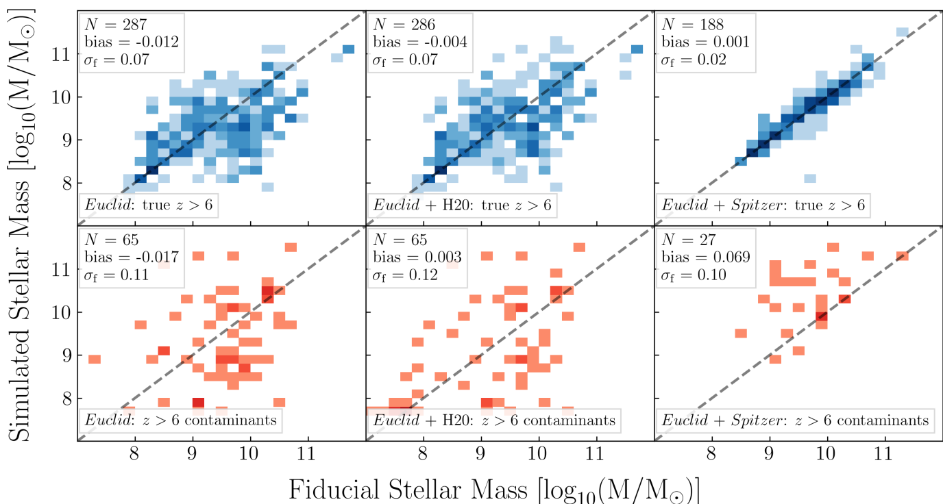
Fig. 11: Fiducial stellar mass versus Euclid (+ancillary) photometry-derived stellar mass for true z > 6 galaxies (upper panels) and z > 6 contaminants (lower panels), for three scenarios of Euclid and ancillary photometry. The number of galaxies shown is indicated in the upper-left corner of each panel, as is the bias and scatter \sigma_f . The bias is defined as mean[(M_{sim} - M_{fid})/M_{fid}] and the scatter as rms[(M_{sim} - M_{fid})/M_{fid}] . The colour intensity corresponds to the number of galaxies in each bin (darker colours correspond to more sources).
