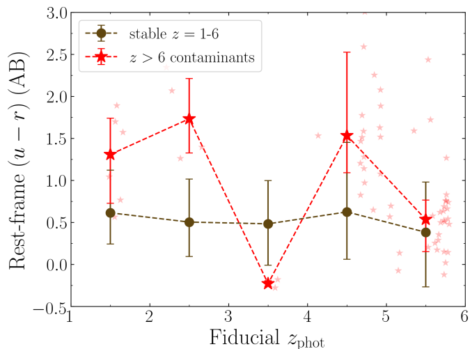
Fig. 8: Rest-frame ( u - r ) colour of the z > 6 contaminants and stable intermediate- z galaxies against the fiducial redshift, based on real COSMOS photometry. The z > 6 contaminants and stable intermediate- z galaxies are identified through Euclid photometry alone. For both populations, we plot the median ( u - r ) colour in \Delta z = 1.0 fiducial redshift bins, where the error bars represent the 16 th and 84 th percentiles. The individual data points of z > 6 contaminants are shown with small red stars.
