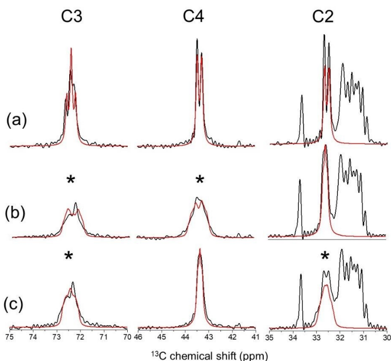
Figure 2. ^{13}\text{C} CP-MAS NMR analysis of rHDL and MLVs containing POPC and 10 mol % [2,3,4-^{13}\text{C}_3] cholesterol. (a) Spectrum of rHDL at a MAS frequency ( \nu_r ) of 9000 Hz overlaid with a simulated spectrum (red) with ^{13}\text{C} - ^{13}\text{C} J -coupling constants of 33 Hz and a line broadening factor of 30 Hz. (b) Spectrum of rHDL at \nu_r = 5113 Hz, which corresponds to the n = 1 rotational resonance condition with respect to the frequencies of C3 and C4 at the applied magnetic field of 16.3 T. (c) Spectrum of rHDL at \nu_r = 7010 Hz, which corresponds to the n = 1 rotational resonance condition with respect to the C2 and C3 frequencies. The blue lines in (b) and (c) are simulated spectra for ^{13}\text{C} - ^{13}\text{C} dipolar coupling constants b_{av}^{23} = b_{av}^{34} = 250 Hz at the two rotational resonance conditions.
