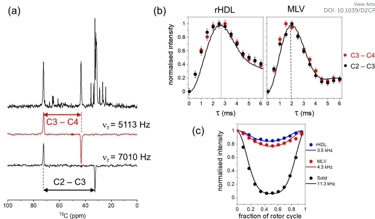
Figure 3. Measurements of ^{13}\text{C} - ^{13}\text{C} and ^{13}\text{C} - ^1\text{H} dipolar couplings for cholesterol in rHDL and MLVs determined by CP-MAS ssNMR. (a) Selective excitation of C2 - C3 and C3 - C4 ^{13}\text{C} - ^{13}\text{C} ZQ coherences at the n = 1 rotational conditions for both spin pairs, detected by conversion of ZQ to DQ coherence and reconversion to observable magnetization. (b) Build-up and decay of C2 - C3 (black circles) and C3 - C4 (red circles) ^{13}\text{C} difference intensities as a function of the ZQ excitation period \tau of the NMR pulse sequence (given in the Supplementary Information, Figure S1a). Solid lines are the best fitting simulated ZQ build-up curves corresponding to the values of dipolar coupling constants b_{av}^{23} and b_{av}^{34} and zero-quantum relaxation time, T_2^{ZQ} , given in the main text. (c) Evolution of the ^{13}\text{C} transverse magnetisation of C3 over one cycle of sample rotation in the presence of C3 - H3 dipolar coupling, measured using the DIPSHIFT experiment (Figure S1b).
