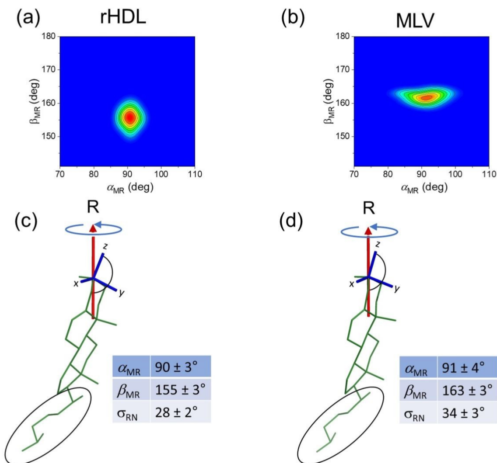
Figure 5. Average orientation in HDL and MLVs of the rigid ring system of cholesterol relative to the principal rotation axis R . (a) and (b) Contour plots showing the combinations of \alpha_{MR} and \beta_{MR} that are consistent with the three measured dipolar coupling values. Full details of the calculation are given in the Experimental section 5.2. (c) and (d) Orientations of cholesterol (and the molecular axis system) relative to the rotational axis R , as specified by the values of \alpha_{MR} and \beta_{MR} corresponding to the red central region of the contour plots. The tables give the ranges of possible angles and standard deviation \sigma_{RN} consistent with the data. The average orientation of the flexible hydrocarbon tail (circled) cannot be determined from the dipolar couplings.
