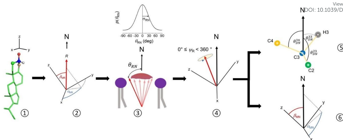
Figure 4. Schematic of the procedure for calculating the orientation of cholesterol relative to the rotational axis. Step 1: A molecular axis system is defined, based on the geometry of cholesterol (see main text for details). Step 2: Angles \alpha_{MR} and \beta_{MR} specify the orientation of the principal rotational axis R of cholesterol in the molecular axis system. Step 3: Cholesterol and its rotational axis undergo random fluctuations from the average position of R along the bilayer normal N by angles \theta_{RN} . The amplitude of deviation from N is defined by a Gaussian distribution with standard deviation \sigma_{RN} . Step 4: The cholesterol molecule in each orientation undergoes rotation about R by angle \psi_{RN} to generate a set of molecular rotamers. Step 5: From each cholesterol orientation are calculated the angles between the ij internuclear vectors and N ( \theta_{DR}^{23} , \theta_{DR}^{34} and \theta_{DR}^{33} ), from which the average values of the dipolar coupling constants are obtained according to Eq. [4]. Step 6: The orientational distribution of cholesterol molecules generated by Steps 3 and 4 is represented by the distribution of angles \alpha_{MN} and \beta_{MN} . Steps 2 to 6 are carried out iteratively to find the values of \alpha_{MR} and \beta_{MR} that are consistent with the experimentally determined values of b_{av}^{ij} .
