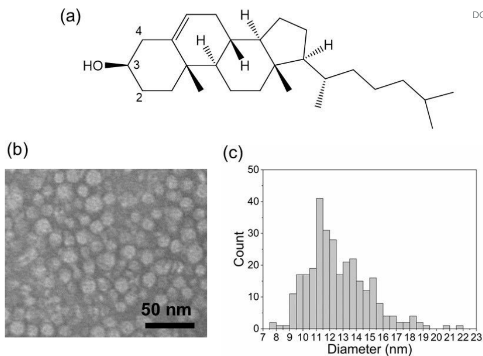
Figure 1. Morphological analysis of rHDL containing [2,3,4- ^{13}\text{C}_3 ]cholesterol. (a) The chemical structure of cholesterol indicating the ^{13}\text{C} -labelled sites, C2, C3 and C4. (b) Negatively-stained TEM image of rHDL. (c) Size distribution of the rHDL nanodiscs measured from the TEM image.
