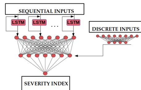
(b) RNN
