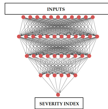
(a) MLP
