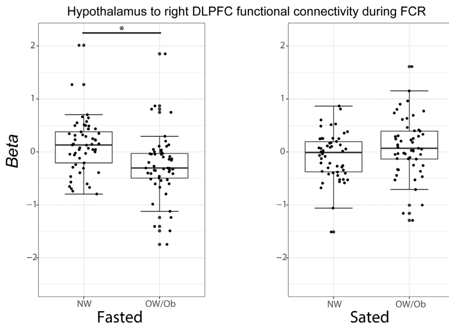
FIGURE 3 Box plot showing hypothalamic functional connectivity (y-axes: beta estimates) to the right dorsolateral prefrontal cortex (DLPFC) in the fasted and sated state during food cue reactivity (FCR) in normal-weight (NW) and overweight/obese (OW/Ob) participants. A two-way interaction between hunger state and body mass index (BMI) group was identified in parts of the right DLPFC ( p_{FWE} < .05 ). In the fasted state, NW participants showed higher functional connectivity between the hypothalamus and the right DLPFC than the OW/Ob group. No group differences were observed in the sated state.
