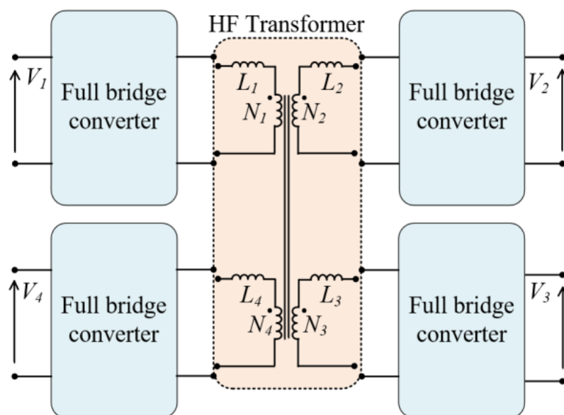
Figure 7. Quadruple-Active-Bridge converter topology.
