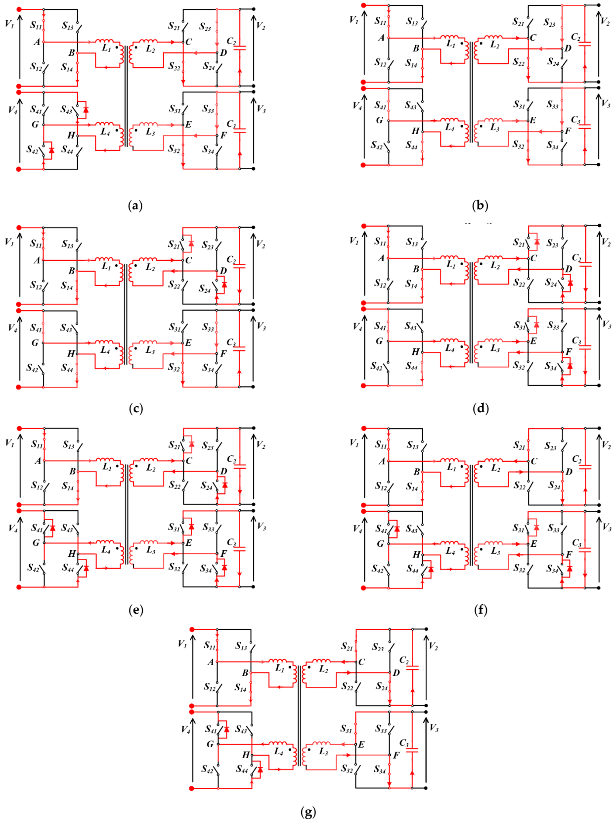
Figure 10. Equivalent circuit of the multi-port DAB converter: (a) time-interval 1 [0 < t < \vartheta_{14}] , (b) time-interval 2 [\vartheta_{14} < t < \vartheta_{12}] , (c) time-interval 3 [\vartheta_{12} < t < \vartheta_{13}] , (d) time-interval 4 [\vartheta_{13} < t < \vartheta_{t1}] , (e) time-interval 5 [\vartheta_{t1} < t < \vartheta_{t2}] , (f) time-interval 6 [\vartheta_{t2} < t < \vartheta_{t3}] , (g) time-interval 7 [\vartheta_{t3} < t < \pi] .
