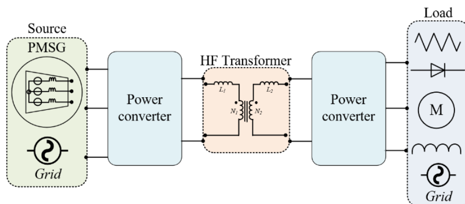
Figure 1. The solid-state transformer concept.
