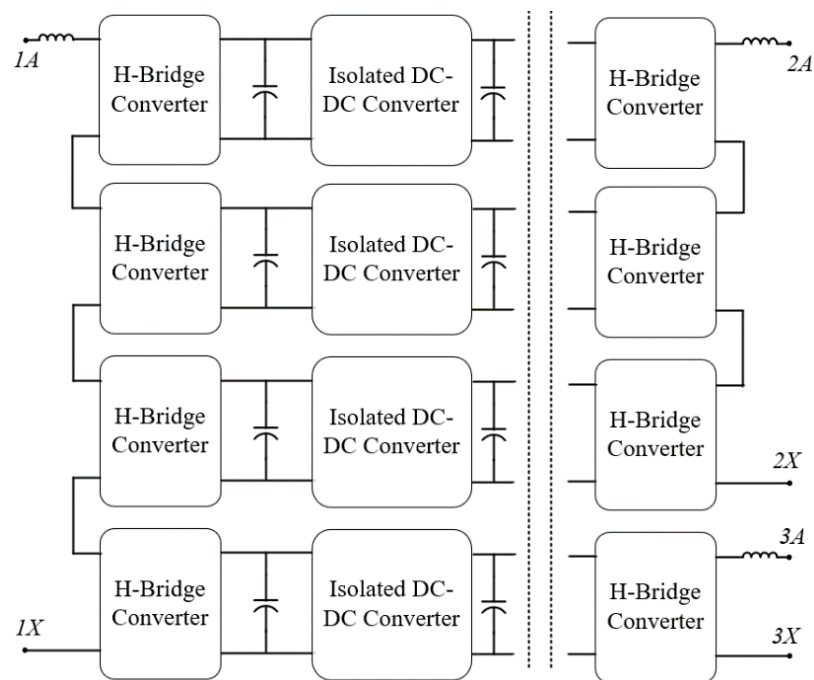
Figure 6. Single-phase representation of the UNIFLEX solid-state transformer topology.
