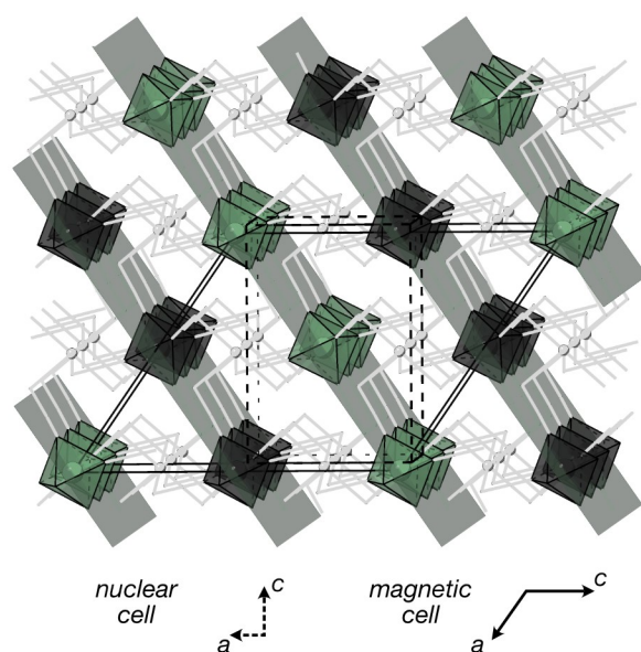
Fig. 4 Magnetic structure of \text{Cr}[\text{Bi}(\text{SCN})_6] \cdot (\text{H}_2\text{O}) . Magnetic Cr atoms are coloured in green and black to illustrate their relative orientations, and the other non-magnetic framework atoms are shown in grey. The \{111\}_{\text{cubic}} type planes in which all spins are ferromagnetically correlated are highlighted. The magnetic and nuclear unit cells are related as follows: \mathbf{a}_{\text{mag}} = \mathbf{a}_{\text{nuc}} - \mathbf{c}_{\text{nuc}} , \mathbf{b}_{\text{mag}} = -\mathbf{b}_{\text{nuc}} and \mathbf{c}_{\text{mag}} = -2\mathbf{a}_{\text{nuc}} .
