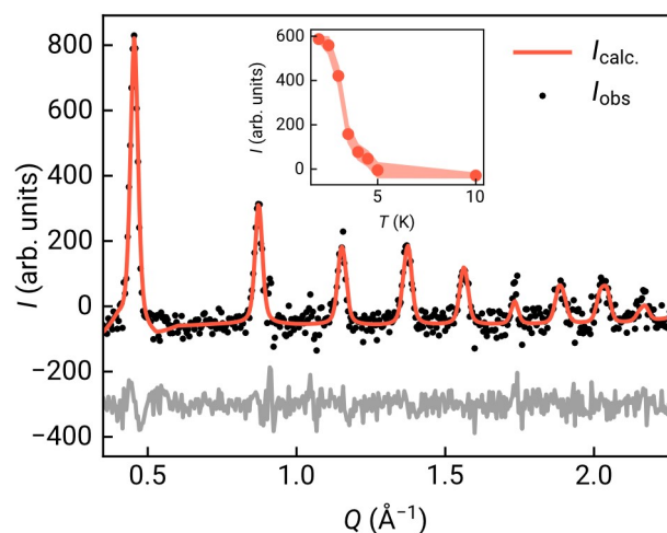
Fig. 3 Detail of the magnetic Rietveld refinement on the Pc_21/n Shubnikov space group, showing all observed magnetic Bragg peaks. The magnetic contribution has been isolated by subtracting the paramagnetic contribution (10 K). Observed (black points) and calculated (orange solid line) powder diffraction pattern (magnetic R_{\text{Bragg}} = 7.77 ). The observed-calculated difference pattern is depicted as a grey line at the bottom of the figure. Inset depicts the temperature dependence of the intensity of the first observed magnetic Bragg line obtained through Gaussian fitting of a single line.
