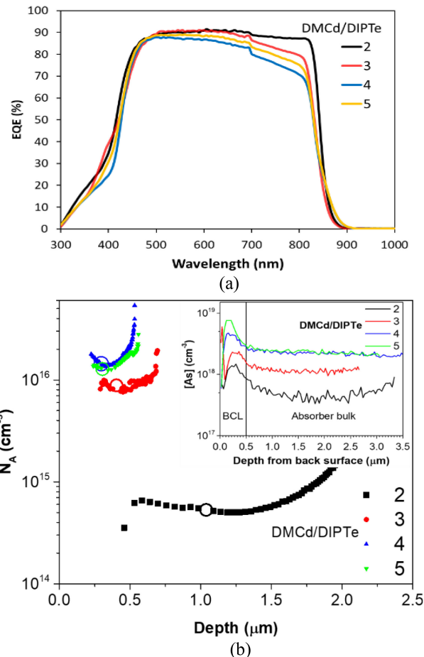
Fig. 10. (a) EQE spectra of Cd-saturated CdTe:As devices. (b) Acceptor concentration ( N_A ) versus depth profiles from varying DMCd/DIPTe partial pressure ratio (inset: Bulk As SIMS depth profiles versus varying DMCd/DiPTE partial pressure ratio). The zero-bias point for each curve is marked with an open circle.
