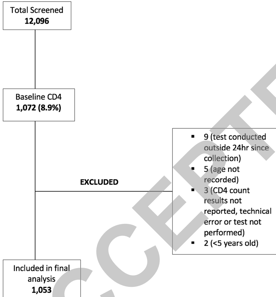
Figure 2. Participants schema
