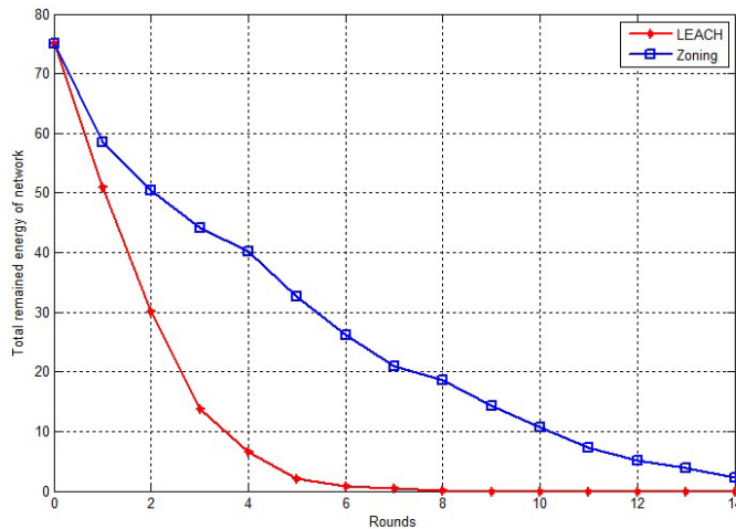
Fig. 1. Total remained energy of network, with n = 150 and \psi=4 .
