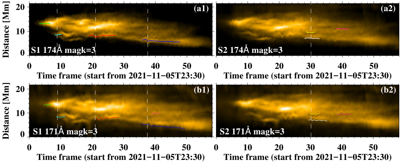
Figure 4. TD maps which display decayless kink oscillations. The dashed lines denote the observation time of HRI images in Fig. ???. The coloured curves indicate the displacement location of centre/edge of corresponding oscillating threads in Fig. ???. The magnification factor is 3 for both data sets.
