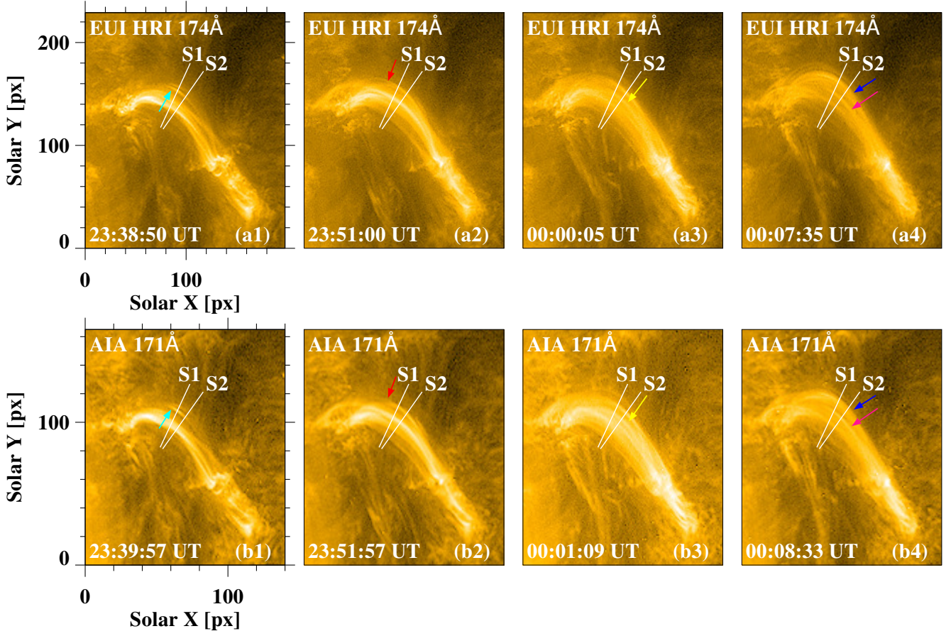
Figure 3. The dynamics of analysed threads. Slits “S1” and “S2” are used to make time–distance (TD) maps in Fig. ???. The coloured arrows denote the oscillating threads which have distinct oscillatory patterns. The images are enhanced to reveal the threads, by applying a high-boost mask.
