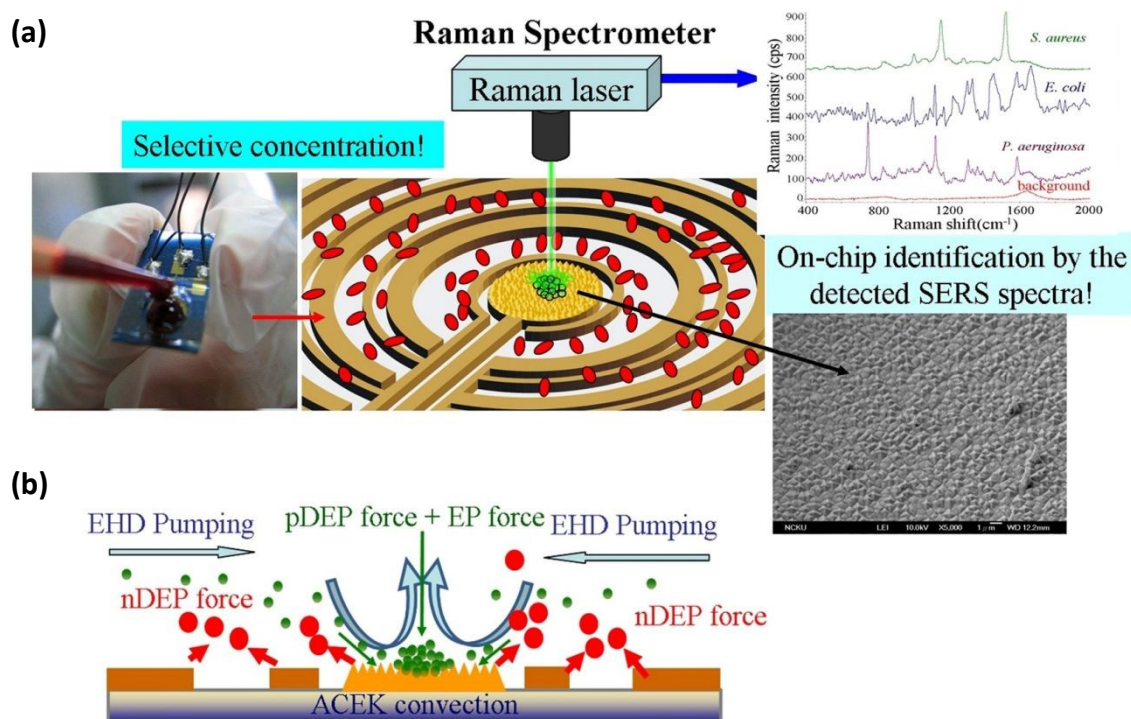
Figure 4. (a) Experimental setup of the DEP SERS-microfluidic platform. The SEM image shows the roughened Au surface at the centre electrode. AC electric field induced electrophoresis (EP) and electro hydrodynamics (EHD) were used to rapidly concentrate bacteria from human blood. SERS Raman spectroscopy fingerprint of the concentrated bacteria identifies the bacteria. (b) Illustration of the hybrid mechanism of selective concentration over a wide range asymmetric electrode array. The image is reprinted from Cheng et al. , 75 Copyright (2013), with permission from Springer Nature.
