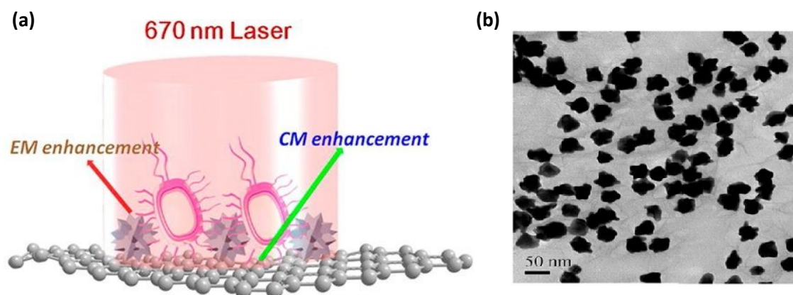
Figure 2. (a) Schematic representation shows the hybrid graphene oxide-based SERS probe for tuning electromagnetic and chemical enhancement simultaneously to detect MRSA . (b) TEM image showing the morphology of the hybrid graphene oxide, where graphene oxide has been attached to nanopopcorn. The image is reprinted from Fan et al. , 56 Copyright (2013), with permission from American Chemical Society.
