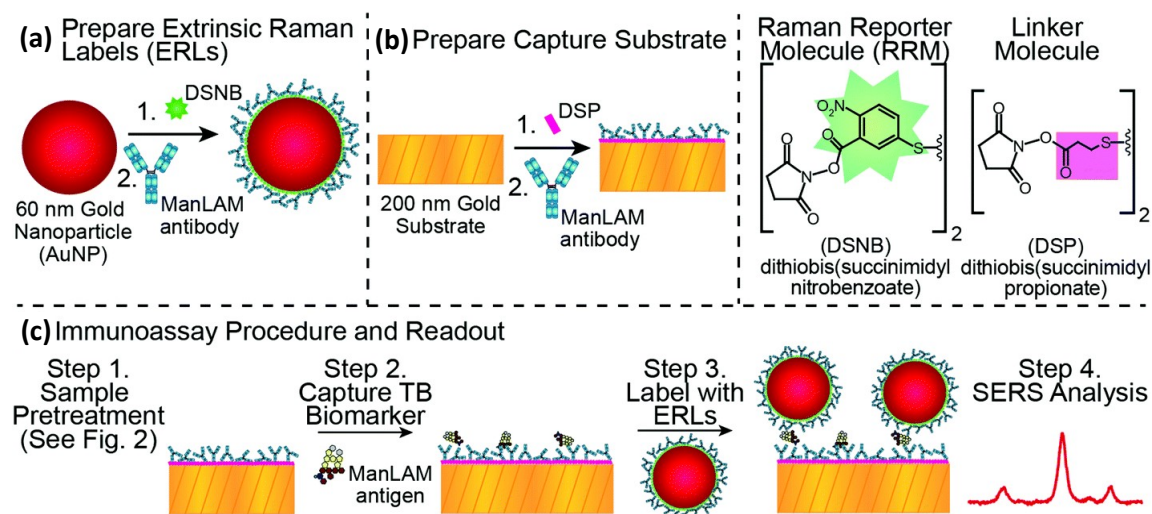
Figure 10. The three main components of the SERS-based immunoassay approach for ManLAM detection: (a) ERL preparation, (b) capture substrate preparation, and (c) major assay steps. The assay is carried out by incubating a pre-treated serum sample (20 \mu L) at room temperature with the capture substrate. The samples are then rinsed, exposed to ERLs (20 \mu L), and analysed by SERS. The image is reprinted from Crawford et al. , 126 Copyright (2017), with permission from Royal Society of Chemistry.
