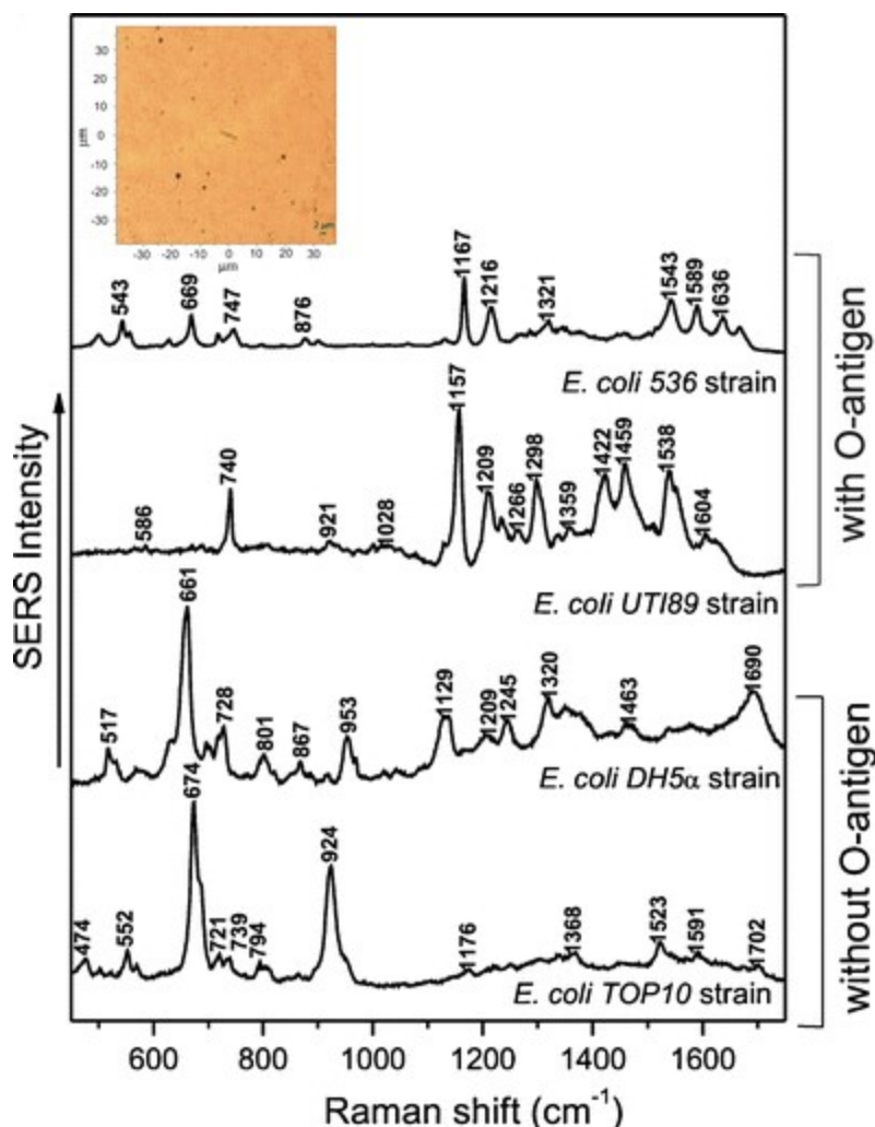
Figure 5. Single-bacterium SERS spectra of rough strains (without O-antigen: DH5 \alpha and TOP10) and of smooth strains (with O-antigen: UTI89, 536), respectively. Inset, microscopic image of the tested E. coli DH5 \alpha rough strain. The image is reprinted from Mircescu et al. , 81 . Copyright (2014), with permission from Springer.
