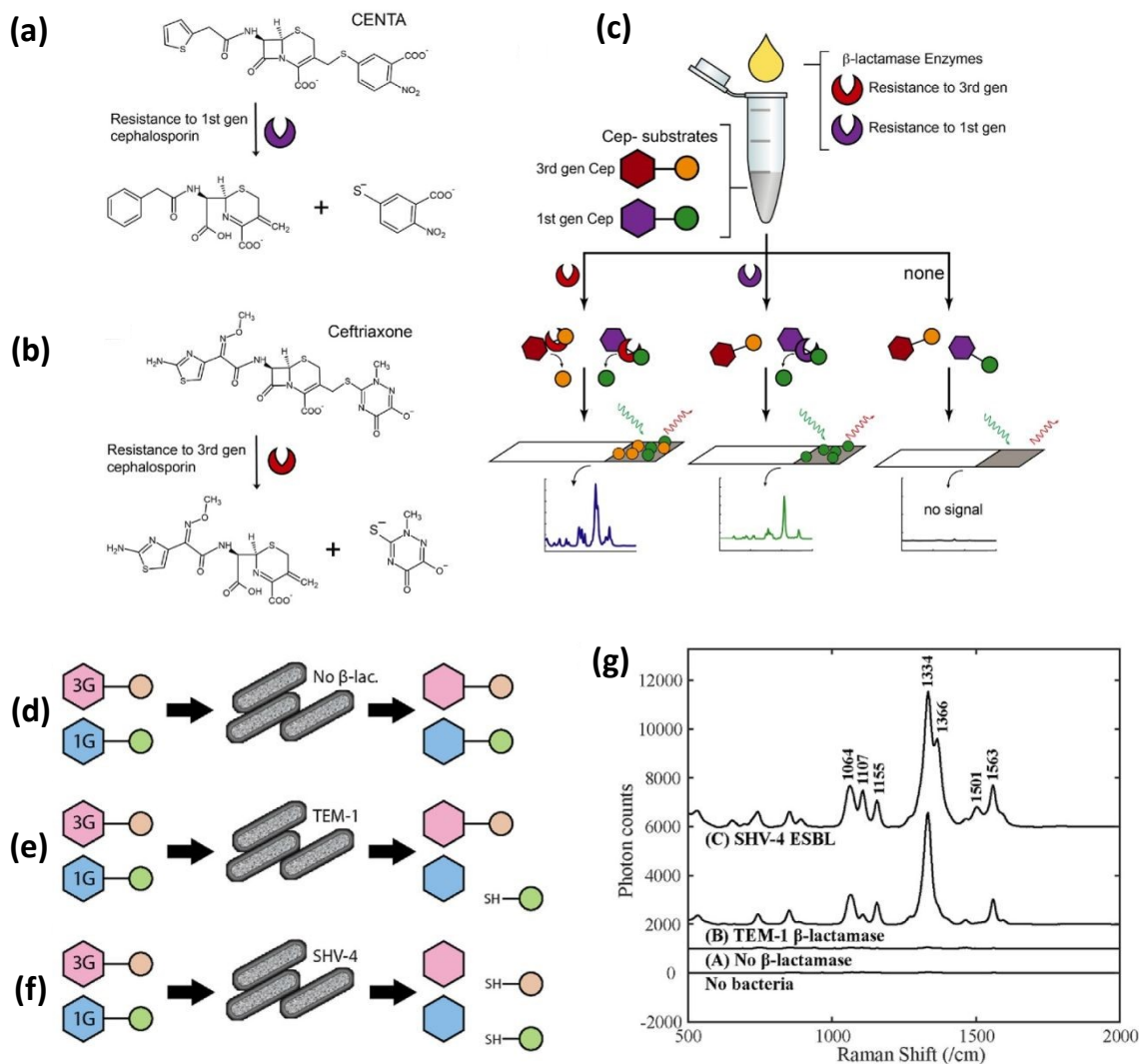
Figure 9. (a) CENTA is hydrolysed by \beta -lactamases that promote resistance to first generation cephalosporins releasing a SERS barcode with a sulfur. (b) CRO is hydrolysed by ESBLs that promote resistance to third generation cephalosporins releasing a SERS barcode with a sulfur. (c) The reporter molecules are combined with a sample containing unknown \beta -lactamases; following incubation, the sample is added to a AgNPs paper SERS sensor. The resulting Raman spectrum indicates which barcodes were released through hydrolysis, thus revealing which generations of cephalosporins will not work against the pathogen. (d) E. coli that does not produce \beta -lactamase will not hydrolyse both reporters. (e) TEM-1 E. coli will hydrolyse the first generation reporter but not the third generation. (f) SHV-4 E. coli will hydrolyse both reporters. (g) SERS spectra show unique signals for the three different strains thus phenotypically differentiating the three strains by their \beta -lactamase activity. The images are reprinted from Hilton et al. , 122 Copyright (2020), with permission from Elsevier.
