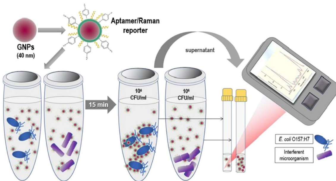
Figure 8. Schematic illustration of the detection mechanism proposed for aptamer-based whole cell detection of E. coli O157:H7. The image is reprinted from Díaz-Amaya et al. , 120 Copyright (2019), with permission from Elsevier.
