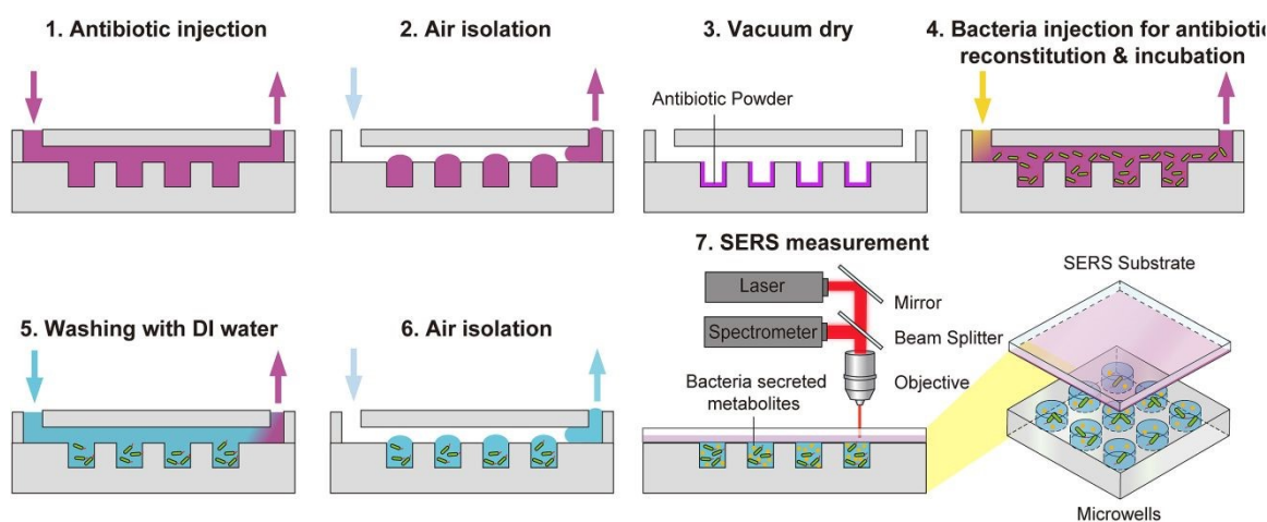
Figure 6. The SERS-AST protocol operated by the automated microfluidic control system. The protocol can be divided into four parts comprising seven steps: (1) “antibiotic preloading”, including antibiotic injection, isolation, and drying (steps 1–3). (2) “bacteria injection for antibiotic reconstitution and incubation” (step 4). (3) “DI water washing and air isolation” (steps 5–6). (4) SERS substrate attachment for multi parallel in-situ “SERS measurement” (step 7). The image is reprinted from Liao et al. , 90 Copyright (2021), with permission from Elsevier.
