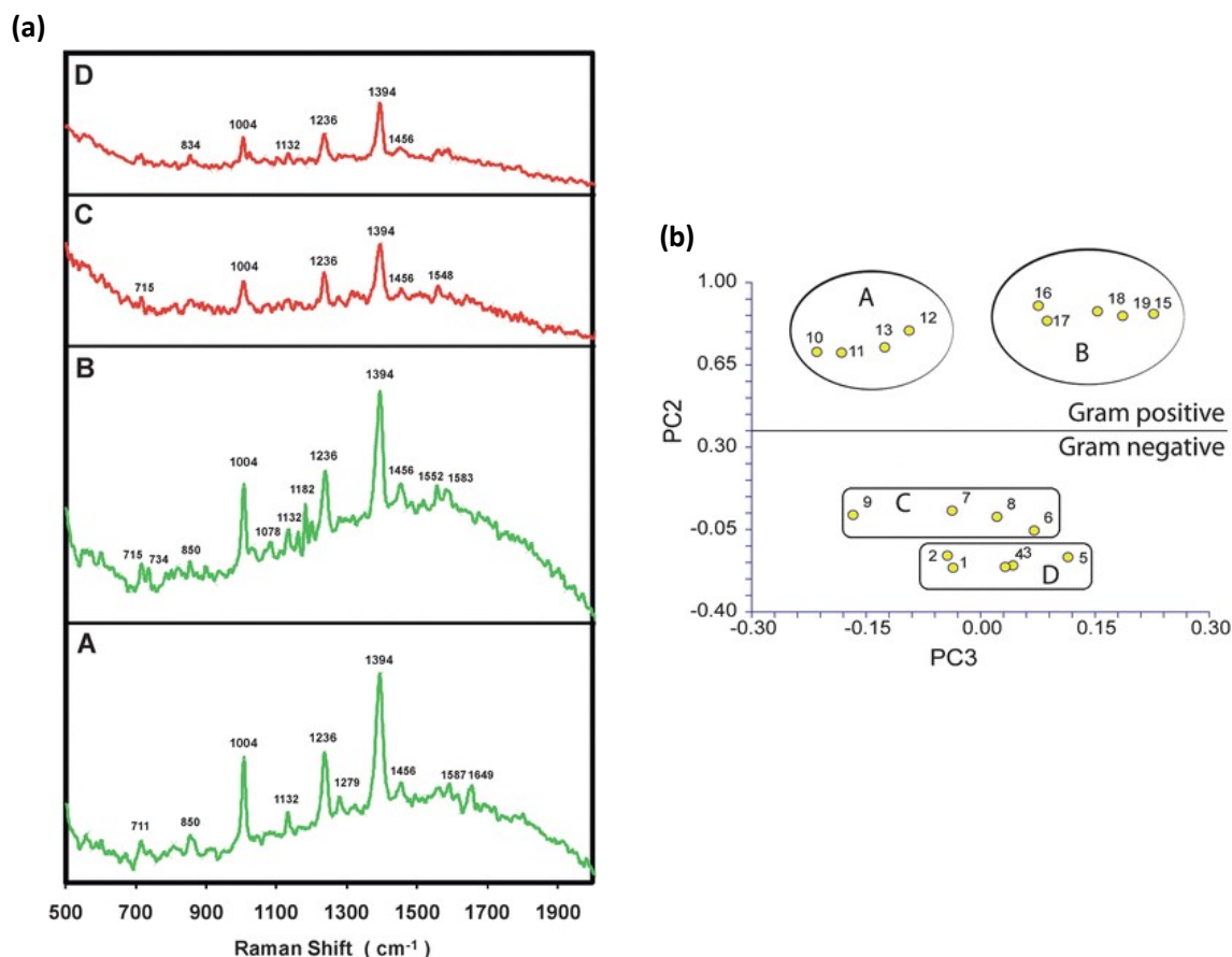
Figure 11. (a) Representative SERS spectra of bacterial lysates: (A) E. faecalis , (B) Streptococcus pyogenes , (C) Acinetobacter baumannii , and (D) K. pneumoniae . (b) Cluster analysis of given Gram-positive and Gram-negative bacteria. The images are reprinted from Pucek et al. , 141 Copyright (2012), with permission from Royal Society of Chemistry.
