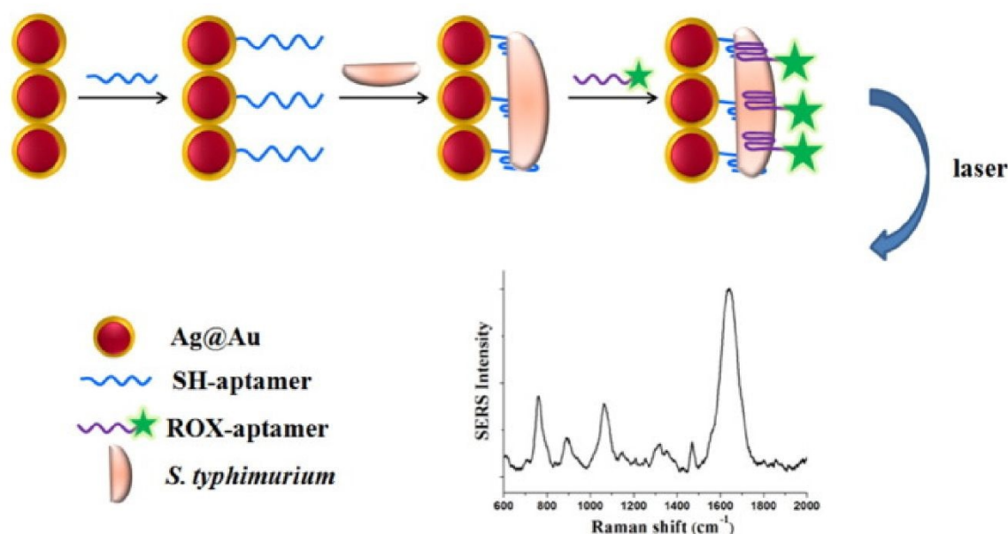
Figure 3. Schematic illustration of SERS-based aptasensor for quantification of S. typhimurium . The image is reprinted from Duan et al. , 64 Copyright (2016), with permission from Elsevier.
