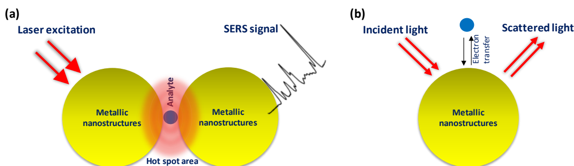
Figure 1. Mechanisms of SERS effect through (a) electromagnetic enhancement of SERS, where analyte is trapped in the hot spot area formed between two adjacent SERS active metallic nanostructures, and (b) electron transfer between SERS active metallic nanostructure and analyte, resulting in chemical enhancement of SERS.
