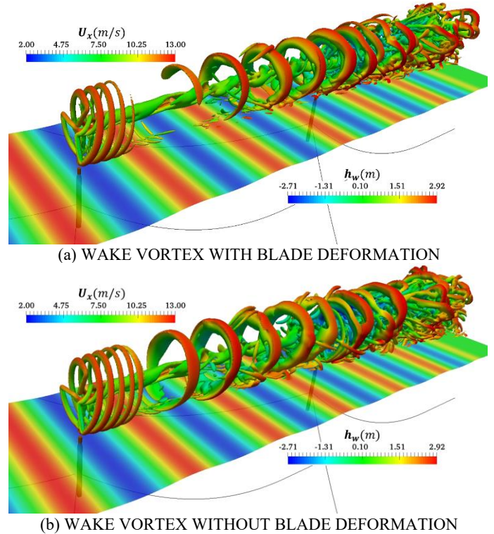
FIGURE 12: WAKE VOETEX STRUCTURE OF TWO TANDEM FOWTS WITH AND WITHOUT BLADE DEFORMATION
