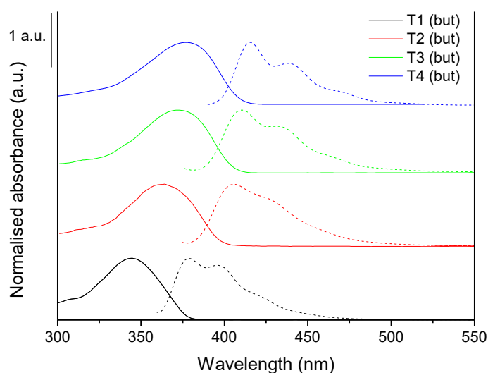
Figure 9. Normalized absorption (continuous line) and emission (dashed line) spectra of the members of the Tn (butyl) family ( 10^{-6} M solutions in 1:2 acetonitrile:benzene).
