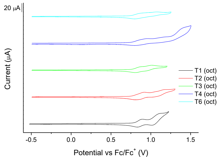
Figure 7. Oxidation waves of the Tn (octyl) series in 1:2 acetonitrile:benzene. The cyclic voltammogram was obtained employing a glassy carbon working electrode, a platinum wire counter electrode and a silver wire reference electrode. All the waves were referenced to ferrocene.
