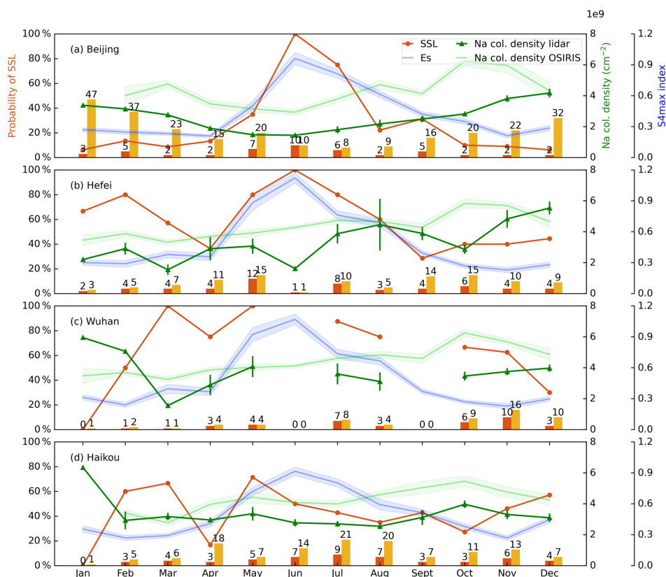
Figure 15. Monthly variations in probability of SSLs per day (orange lines), E_s layer intensity represented by S4_{max} at the height of 95–97 km (blue lines), and Na column number density between 76 and 106 km from OSIRIS (light green lines) and Na lidars (dark green lines) in 2011/2012, at (a) Beijing, (b) Hefei, (c) Wuhan, and (d) Haikou. The orange and yellow bars in the histogram exhibit the number of SSL nights and total nights measured by lidars. The standard errors of the metallic ion density are represented by the width of the blue shaded area. The standard errors of the monthly Na column number density from OSIRIS and Na lidars are represented by the width of the light green shaded area and the dark green bars. The standard error was calculated from the standard deviations of monthly mean divided by the square root of the number of points in each month.
