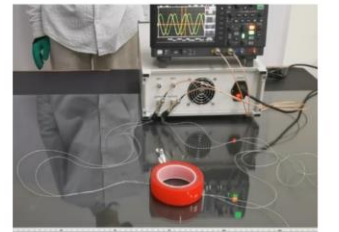
(d) Photograph of the prototype going through the load capacity test
