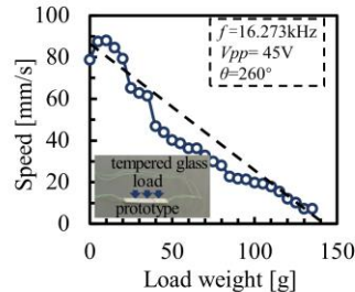
(c) The relationship between the motion speed with the load mass ( V_{pp}=45V , f=16.273kHz , \theta=260^\circ )
