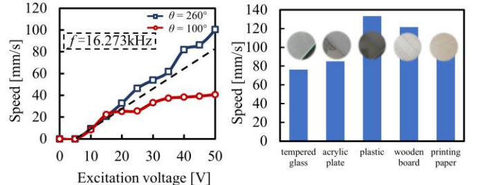
(a) The relationship between the motion speed with the driving voltage on the pure TW points (running on tempered glass, f=16.273kHz )
