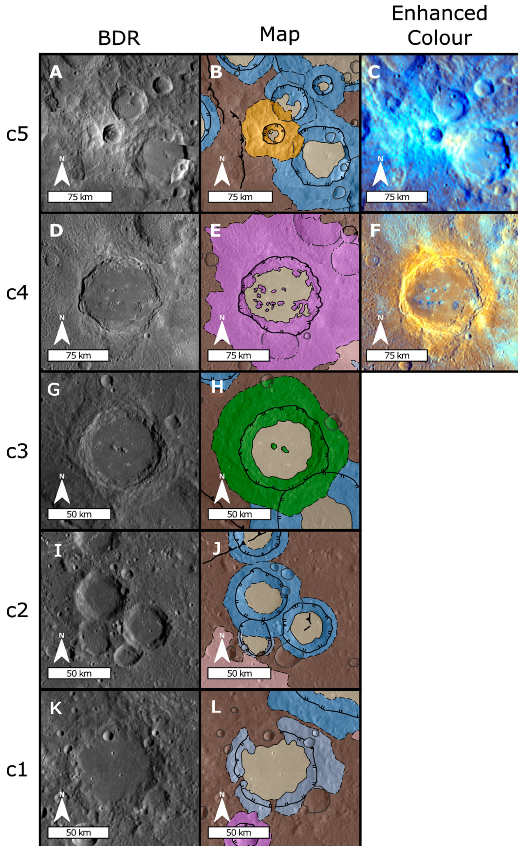
Figure 2. Examples of the 5-class crater degradation states. A, D, G, I and K show the craters in the BDR basemap. B, E, H, J and L show them as mapped. C and F show c5 and c4 craters in enhanced colour, because the presence or absence of albedo rays is the key distinguisher between these crater classes. Albedo features are not used to distinguish between any other crater classes.
