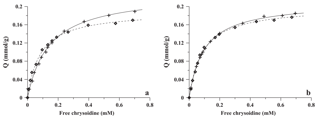
Figure 3 Amount of sorbed chrysidine per unitary weight of sorbent. Q is reported as a function of free chrysidine at equilibrium: (a) FG at pH 4 (+), GG at pH 4 (◇), (b) FG at pH 7 (+), GG at pH 7 (◇).
