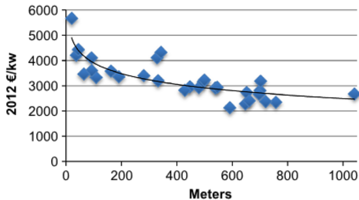
Fig. 3. Relation between net head and CAPEX in our data sample.
