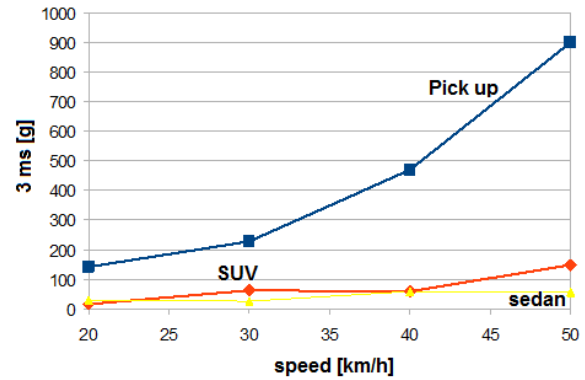
Figure 13: comparison Pick up – SUV and sedan in the side impact
